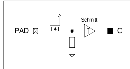
Figure 66 Digital Input with Schmitt Trigger and Pull-Down
