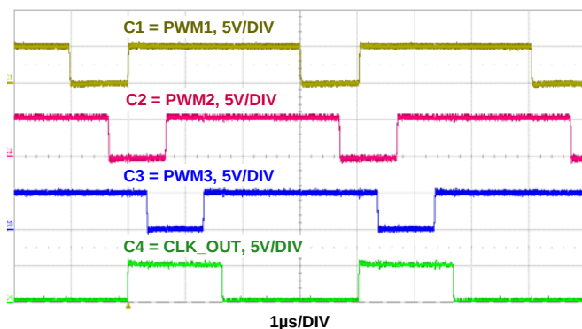
FIGURE 9. WAVEFORMS WITH PWM_INV = V_{CC}
