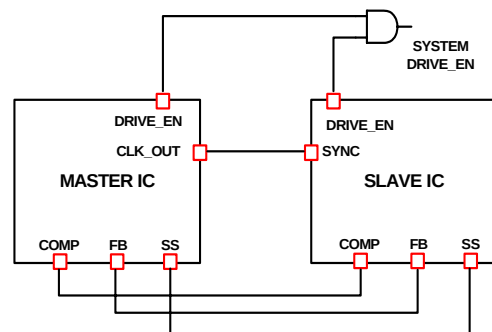
FIGURE 1. CONFIGURATIONS FOR DUAL IC OPERATION
