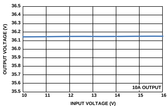
FIGURE 5. OUTPUT VOLTAGE vs INPUT VOLTAGE
