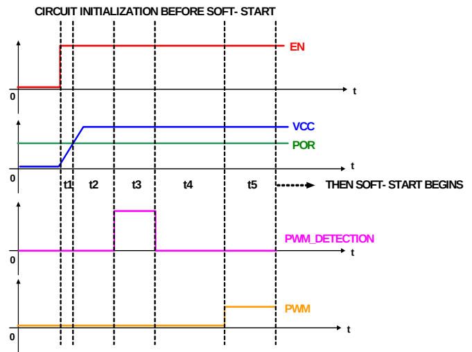
FIGURE 14. CIRCUIT INITIALIZATION BEFORE SOFT-START
