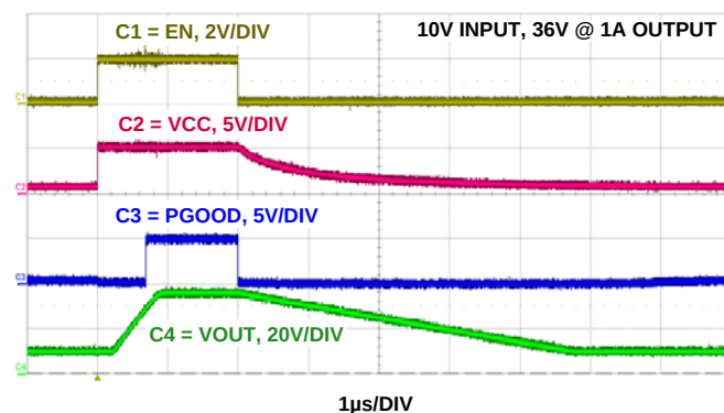
FIGURE 11. ENABLE/DISABLE WAVEFORMS
