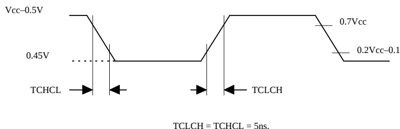
Figure 20. Clock Signal Waveform for ICC Tests in Active and Idle Modes.
