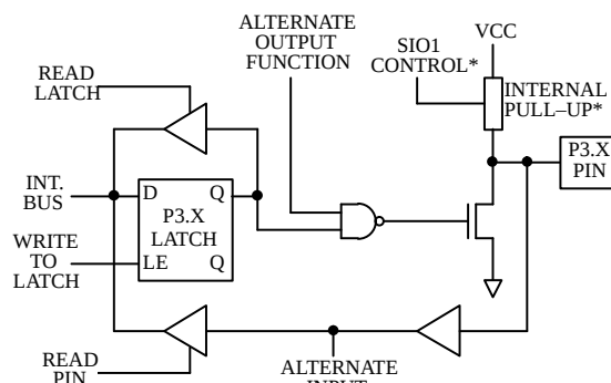
PORT 3 BIT
