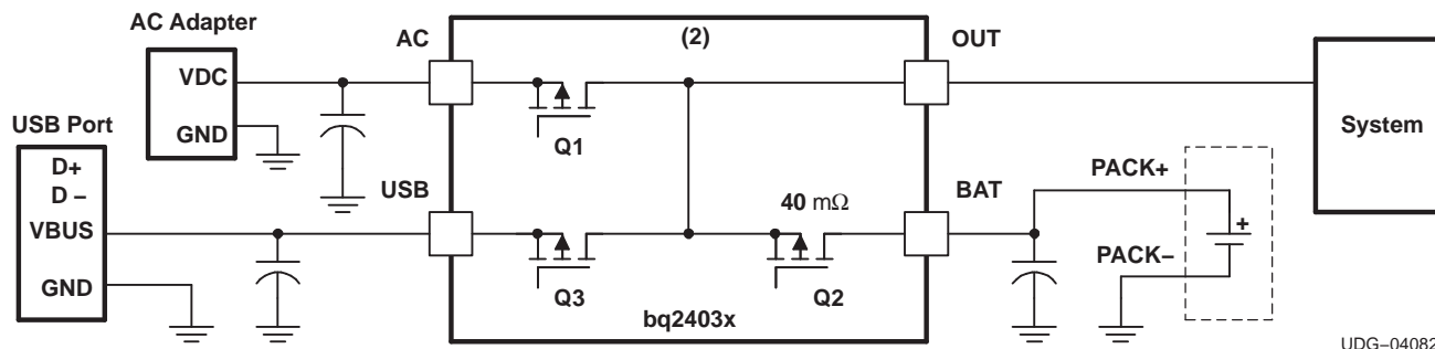
Figure 4. Power-Path Management
