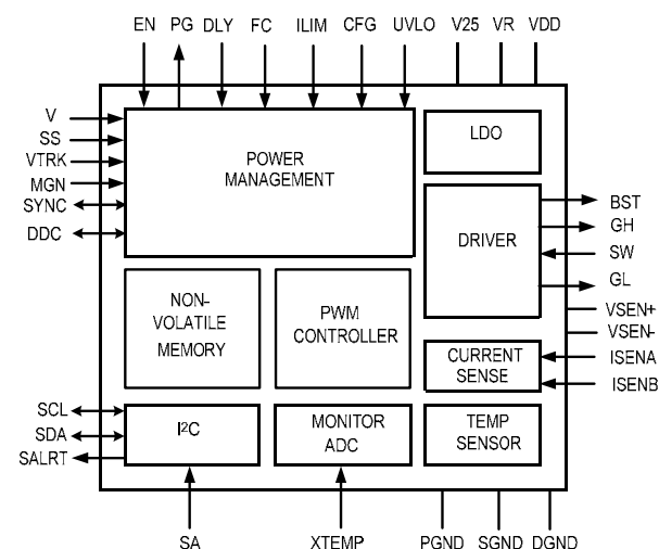
Figure 1. Block Diagram
