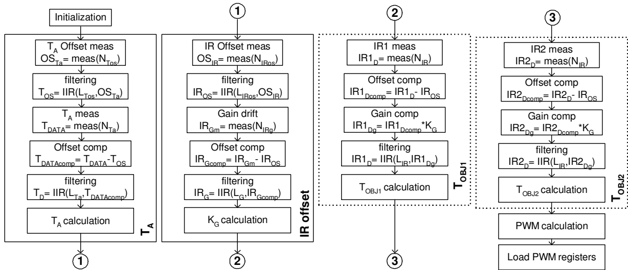
Figure 20: Software flow
