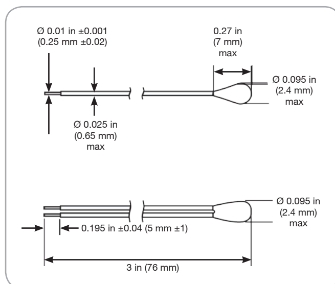
NTC Interchangeable Type TK95 dimensions
