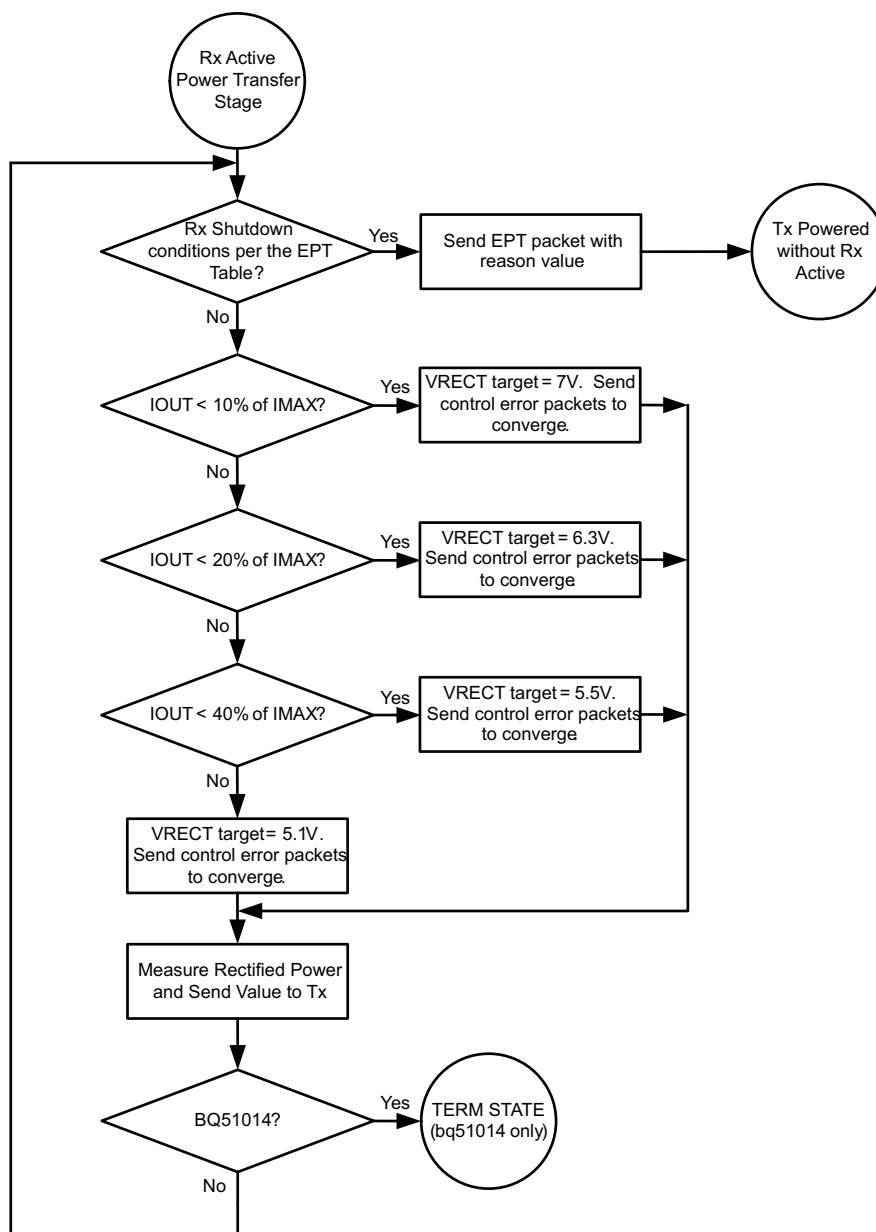
Figure 30. Active Power Transfer Flow Diagram
