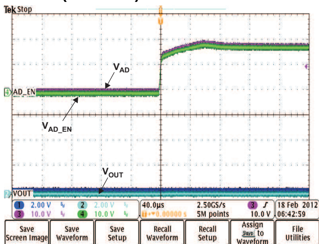
Figure 21. 20V adapter Insertion with AD OVP Enabled (bq51014) and Wireless Power not Present
