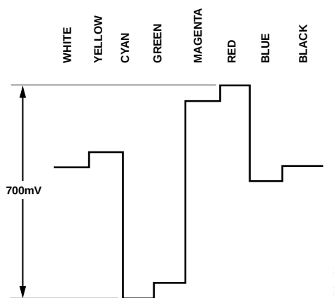
Figure 122. Pr Levels—PAL
