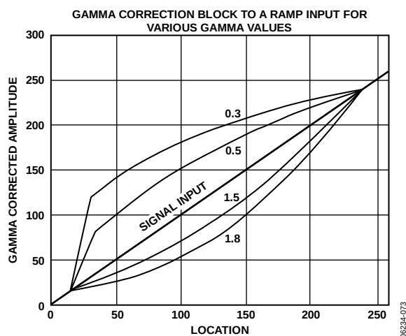
Figure 72. Signal Input (Ramp) and Selectable Output Curves
