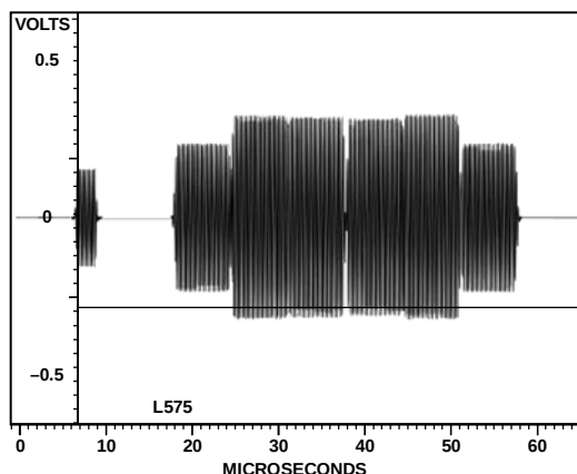
Figure 136. PAL Luma
