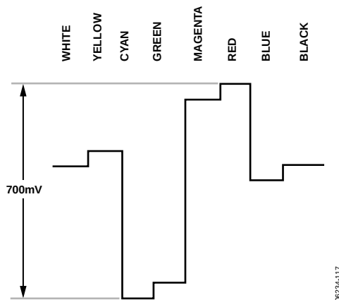
Figure 119. Pr Levels—NTSC
