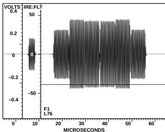
Figure 133. NTSC Luma
