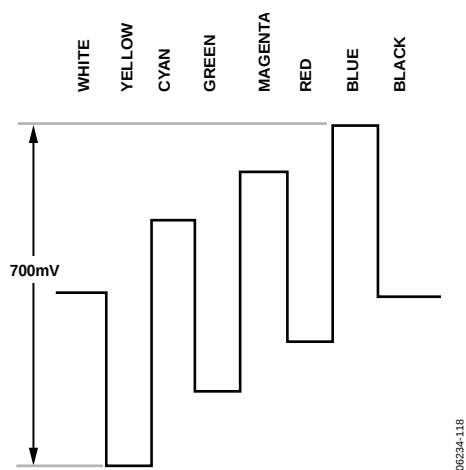
Figure 120. Pb Levels—NTSC
