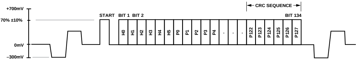
Figure 100. Enhanced Definition (525p) CGMS Type B Waveform
