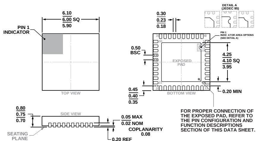
Figure 148. 40-Lead Lead Frame Chip Scale Package [LFCS] 6 mm x 6 mm Body and 0.75 mm Package Height (CP-40-9) Dimensions shown in millimeters
