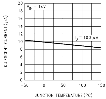
Quiescent Current
