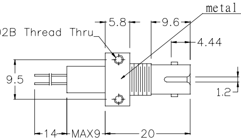
(2)#2-56 UNC02B Thread Thru
