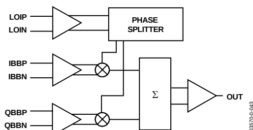
Figure 42. Block Diagram
