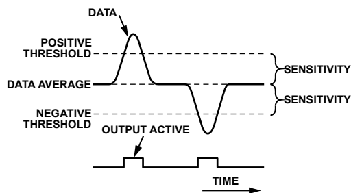
Figure 31. Threshold Sensitivity
