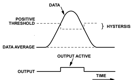
Figure 32. Threshold Hysteresis
