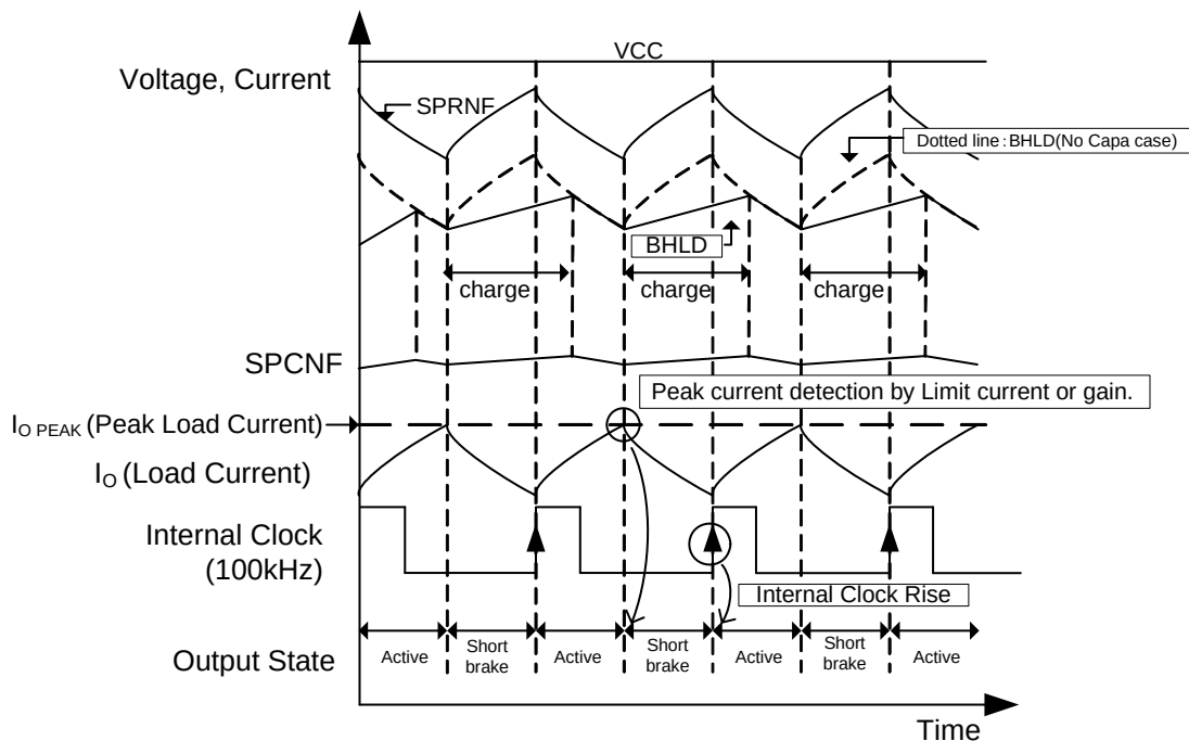
Figure 21. Spindle Driver Operation Timing Chart
