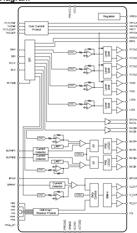
Figure 3. Block diagram
