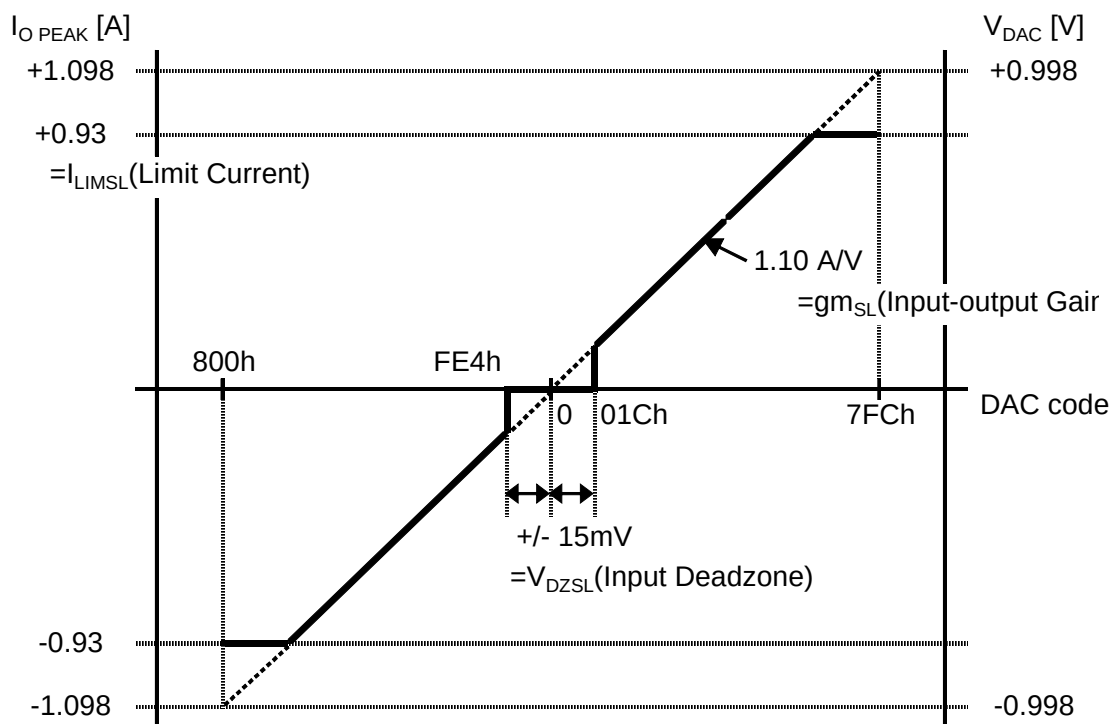
Figure 12. I_{O\text{ PEAK}} Characteristics (When set as R_{\text{SLRNF}}=0.56 \Omega ).
