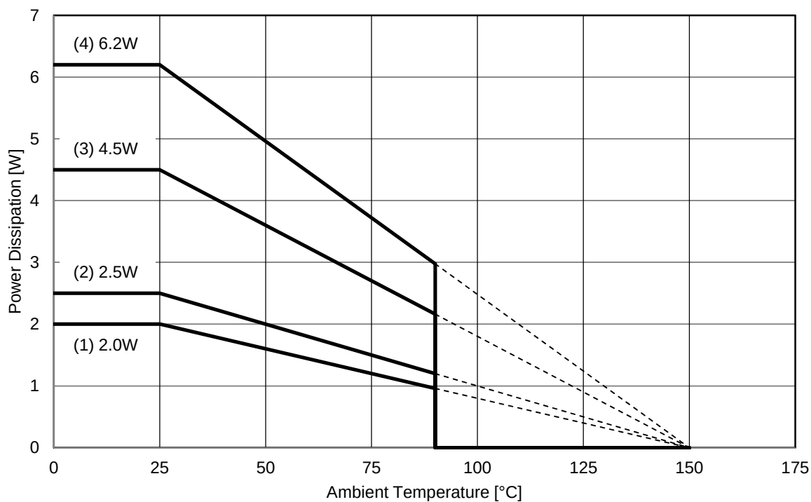
Figure 35. Power dissipation
