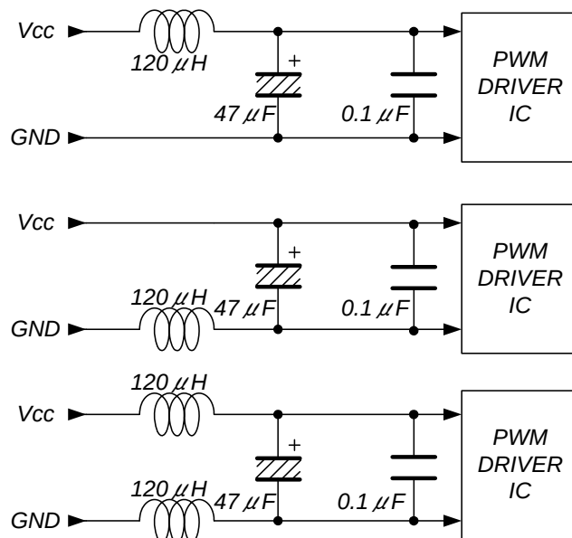
Figure 30. LC Filter Diagram
