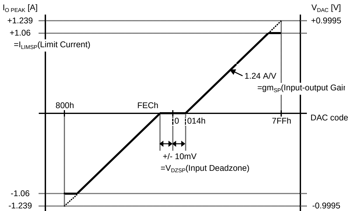
Figure 13. I_{O\text{ PEAK}} Characteristics (When set as R_{\text{SPRNF}}=0.33\ \Omega ).
