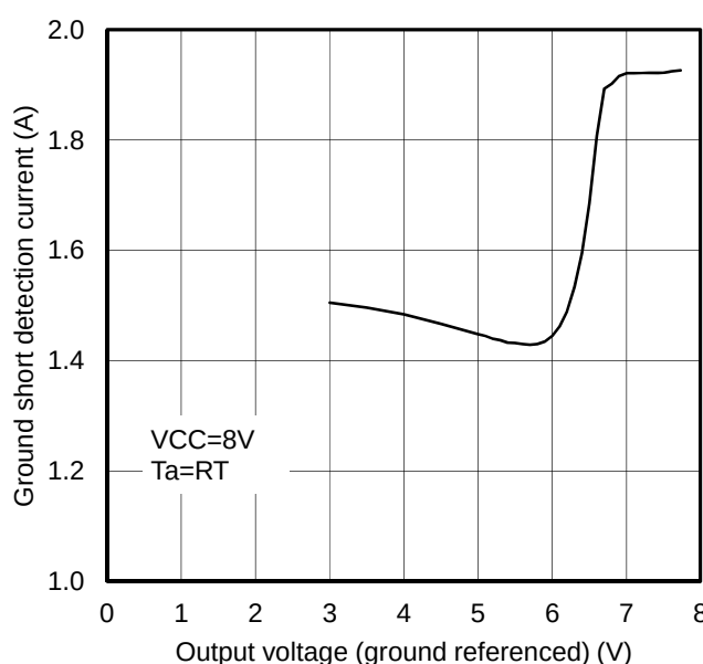
Figure 25. Output voltage vs Ground short detection current
