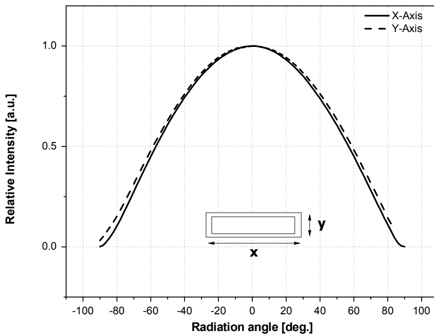
Fig 2. Radiant Pattern, T_a = 25^\circ\text{C} , I_F = 20\text{mA}
