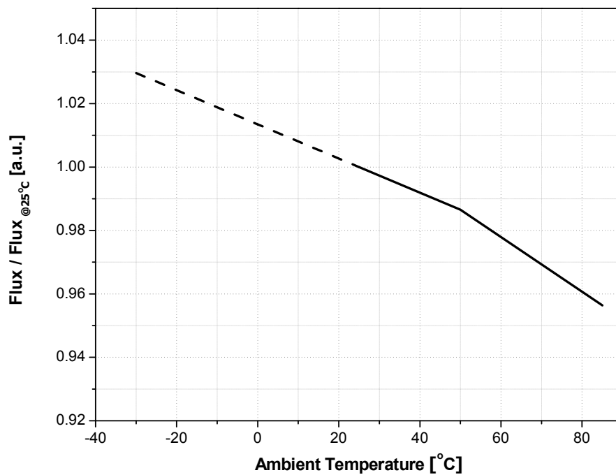
Fig 8. Relative Luminous Flux vs. Ambient Temperature, I_F = 20\text{mA}
