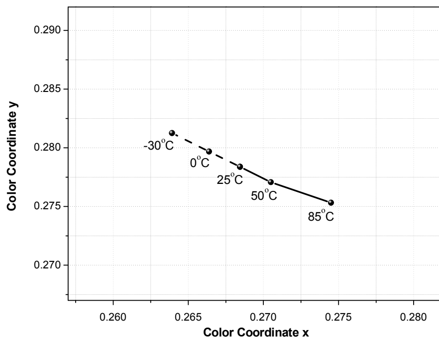
Fig 6. Color Coordinate vs. Ambient Temperature, I_F = 20\text{mA}
