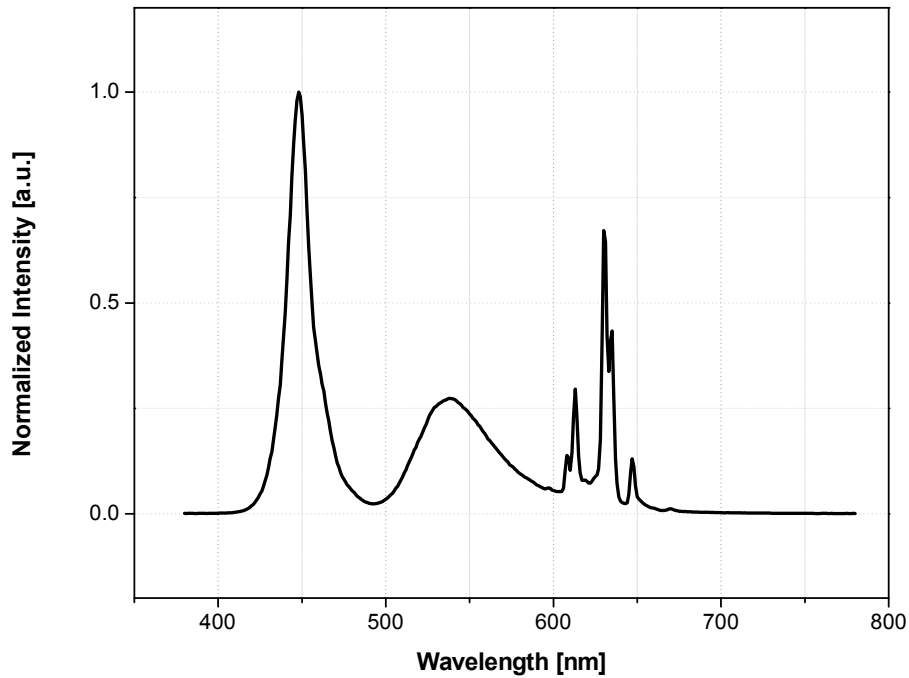
Fig 1. Color Spectrum, T_a = 25^\circ\text{C} , I_F = 20\text{mA}
