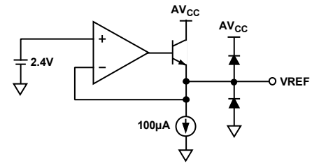
Figure 36. 2.4 V Reference
