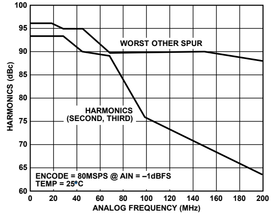
Figure 13. Harmonics vs. Analog Frequency (IF)
