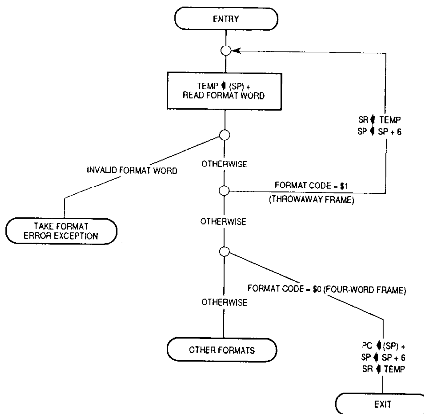
Figure 6-7. RTE Instruction for Throwaway Four-Word Frame
