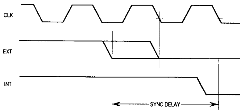
Figure 5-1. Relationship between External and Internal Signals
