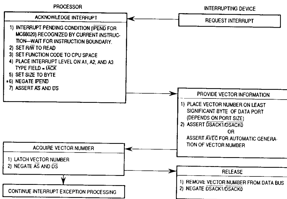
Figure 5-32. Interrupt Acknowledge Cycle Flowchart
