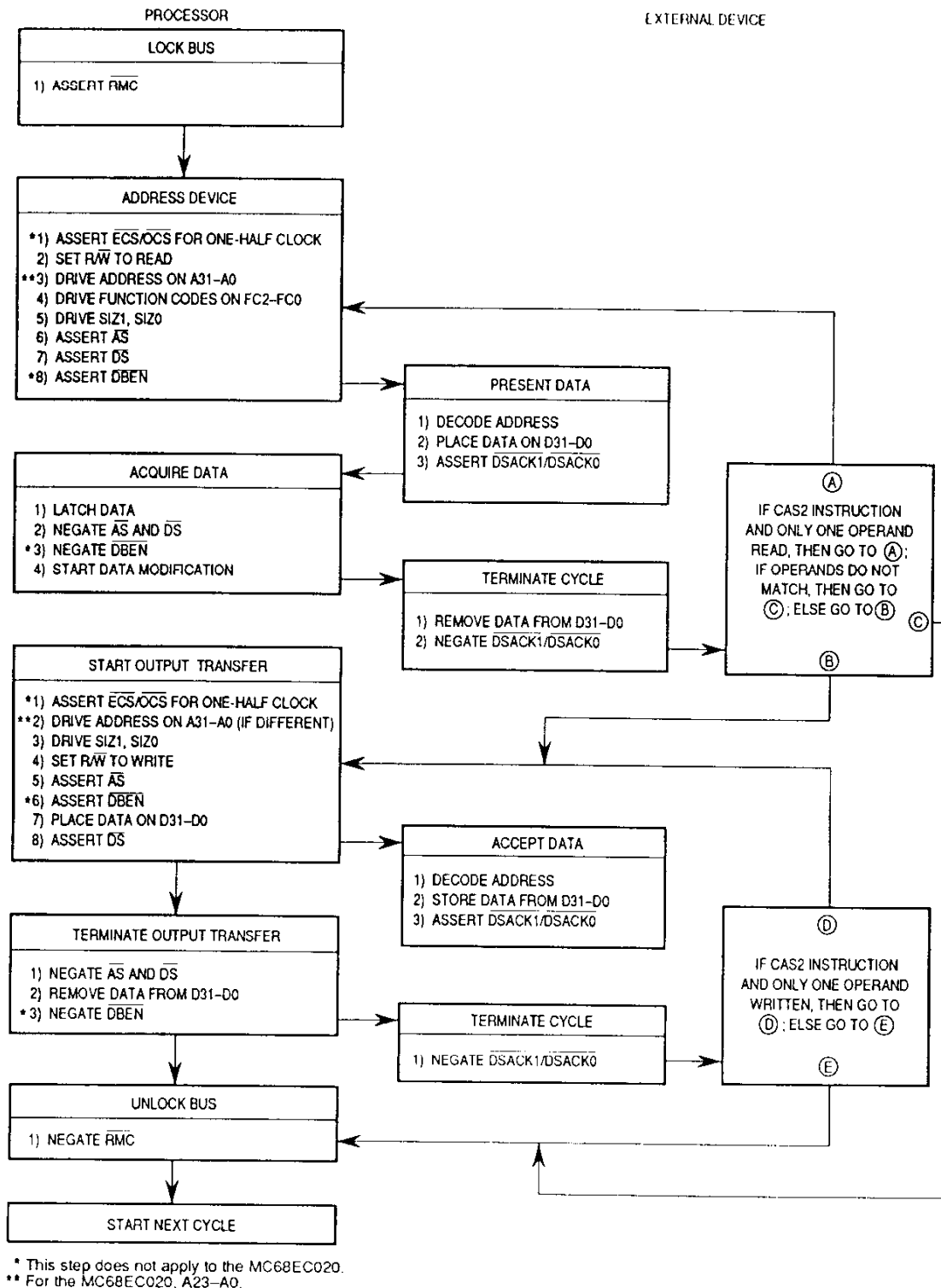
Figure 5-29. Read-Modify-Write Cycle Flowchart
