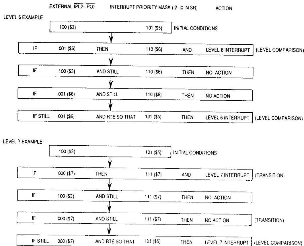
Figure 6-3. Interrupt Recognition Examples
