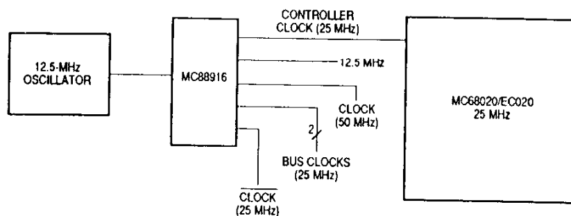
Figure 9-7. High-Resolution Clock Controller
