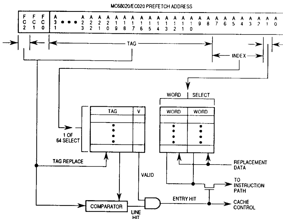
Figure 4-1. MC68020/EC020 On-Chip Cache Organization
