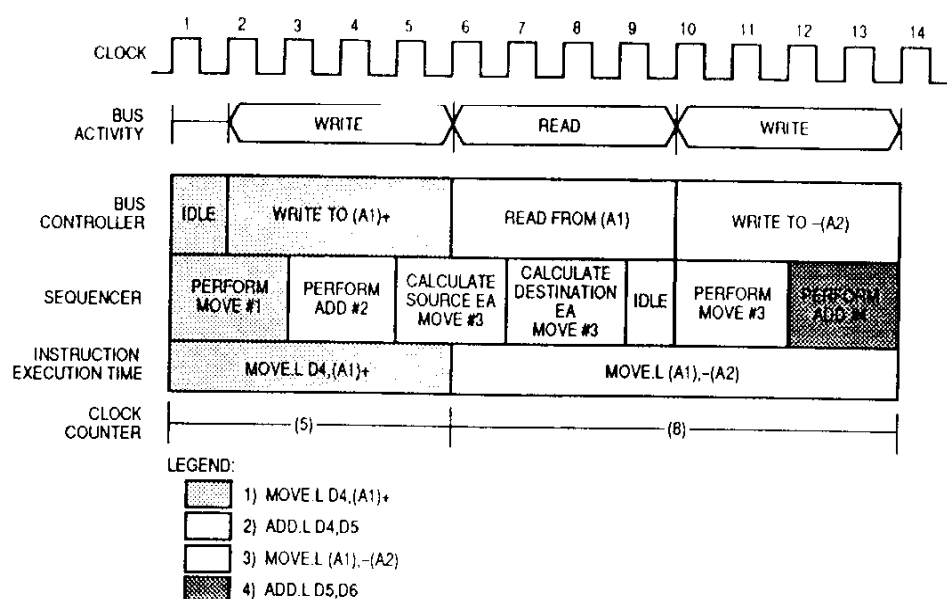
Figure 8-6. Processor Activity for Example 4
