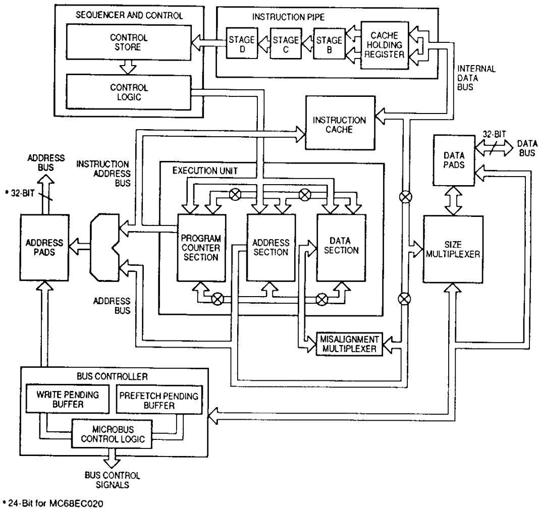
Figure 1-1. MC68020/EC020 Block Diagram
