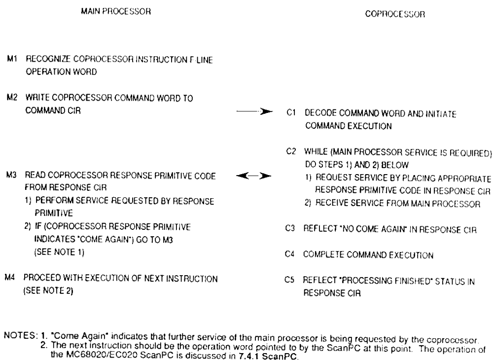
Figure 7-7. Coprocessor Interface Protocol for General Category Instructions
