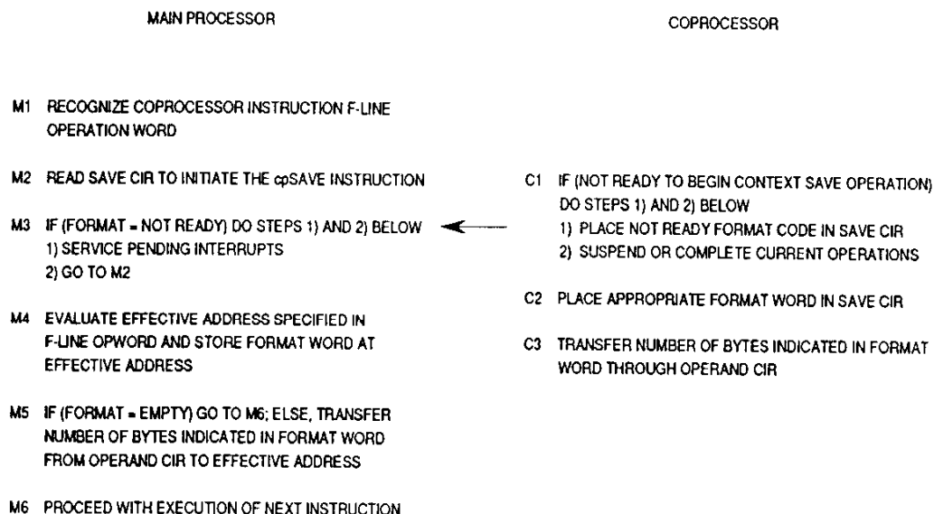
Figure 7-16. Coprocessor Context Save Instruction Protocol
