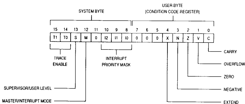
Figure 1-4. Status Register (SR)
