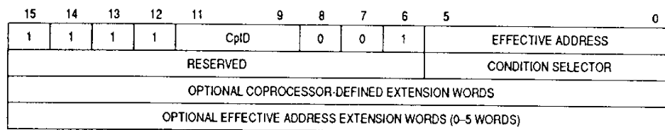
Figure 7-11. Set on Coprocessor Condition Instruction Format (cpScc)
