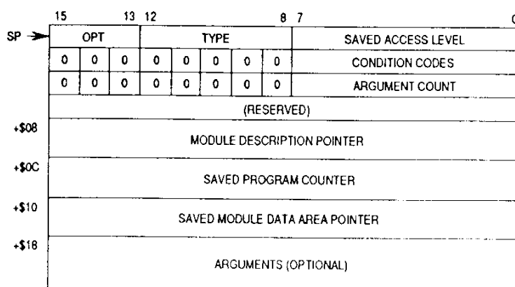
Figure 9-12. Module Call Stack Frame
