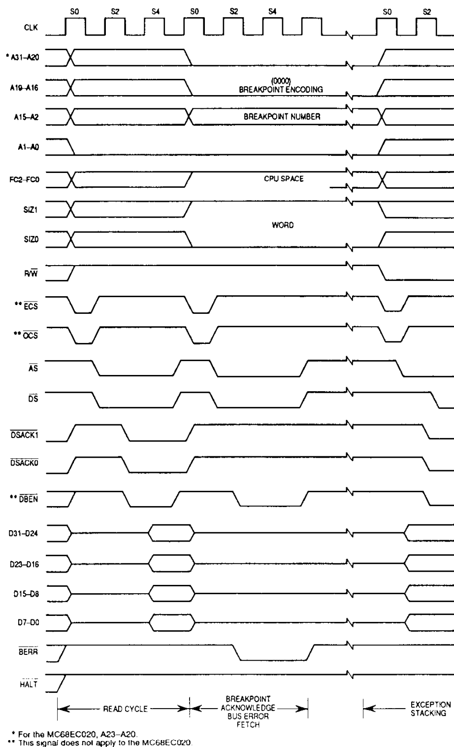
Figure 5-38. Bus Error without DSACK1/DSACK0
