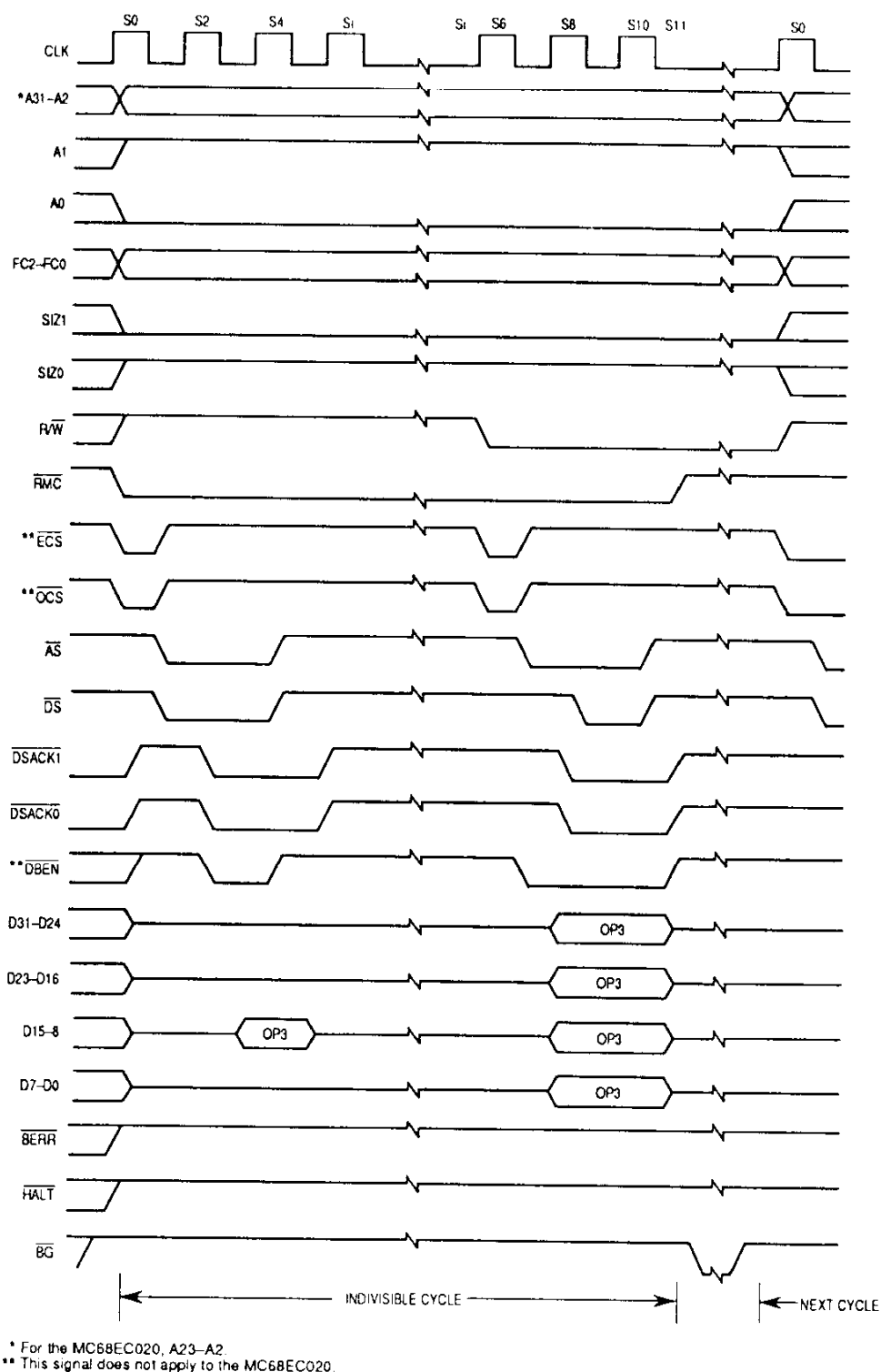
Figure 5-30. Byte Read-Modify-Write Cycle—32-Bit Port (TAS Instruction)
