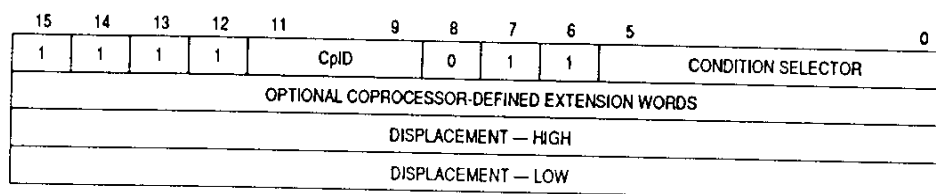
Figure 7-10. Branch on Coprocessor Condition Instruction Format (cpBcc.L)
