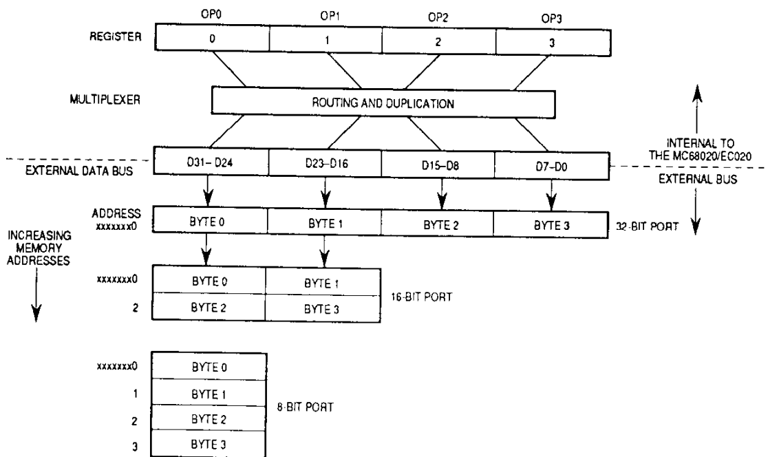
Figure 5-4. MC68020/EC020 Interface to Various Port Sizes
