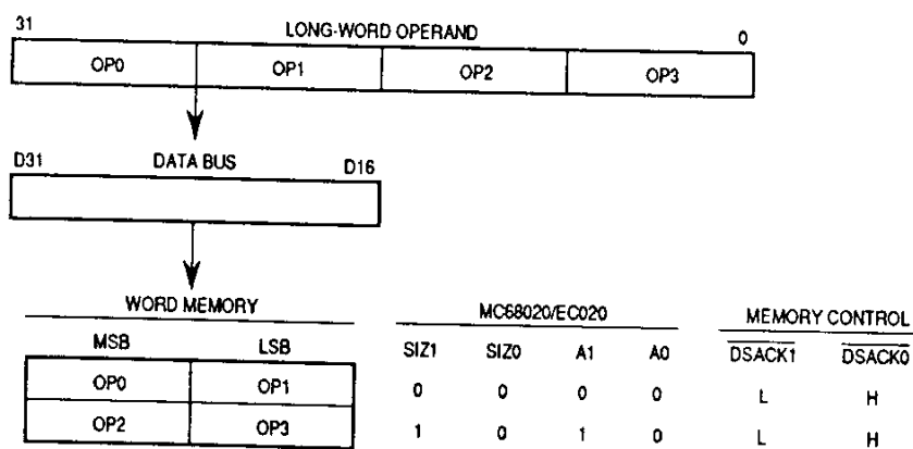
Figure 5-5. Long-Word Operand Write to Word Port Example
