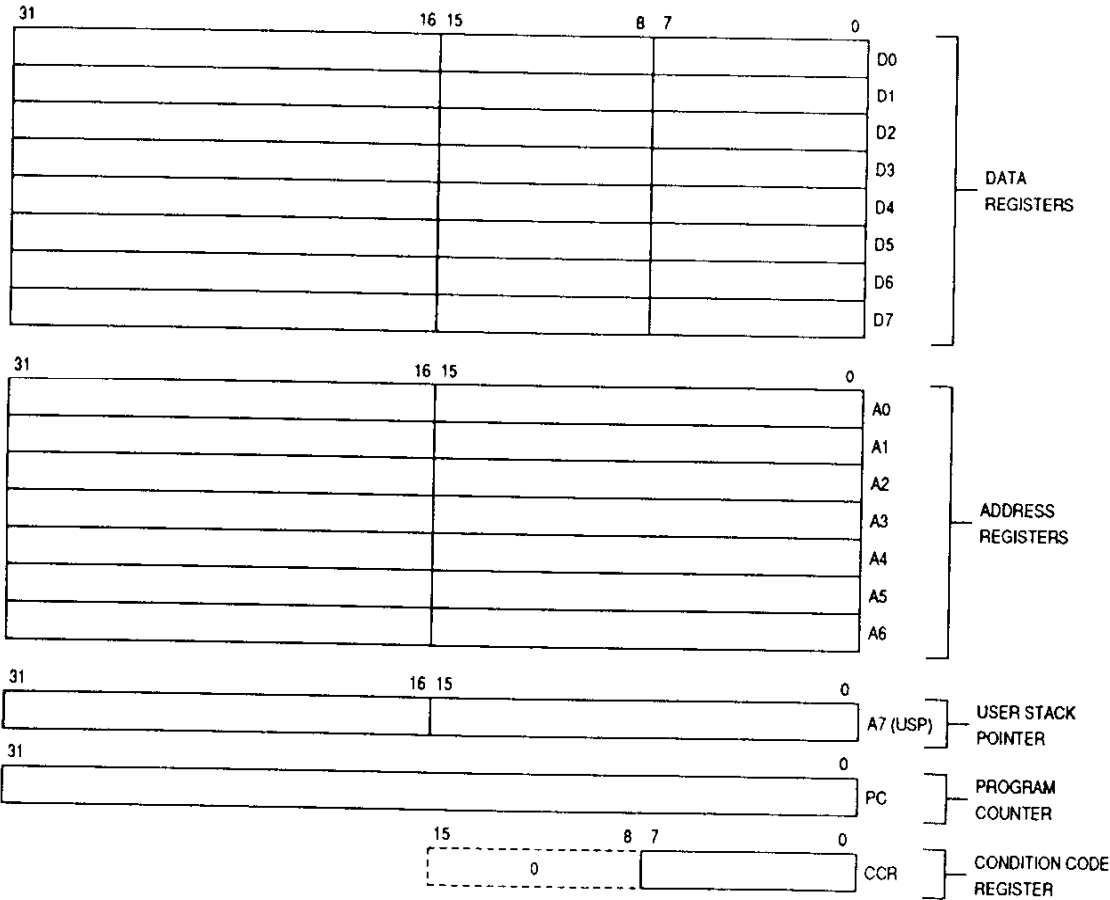
Figure 1-2. User Programming Model
