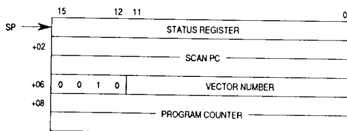
Figure 7-45. MC68020/EC020 Postinstruction Stack Frame
