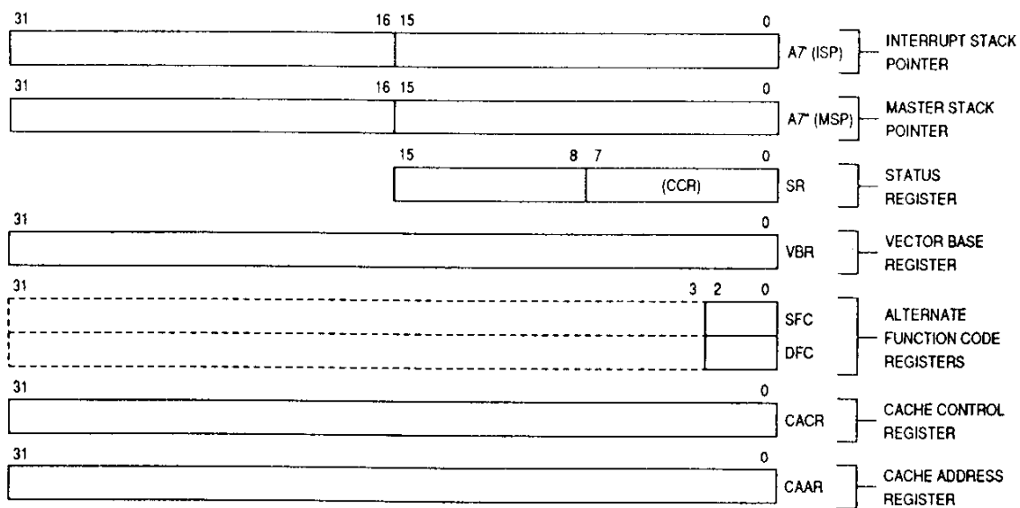
Figure 1-3. Supervisor Programming Model Supplement
