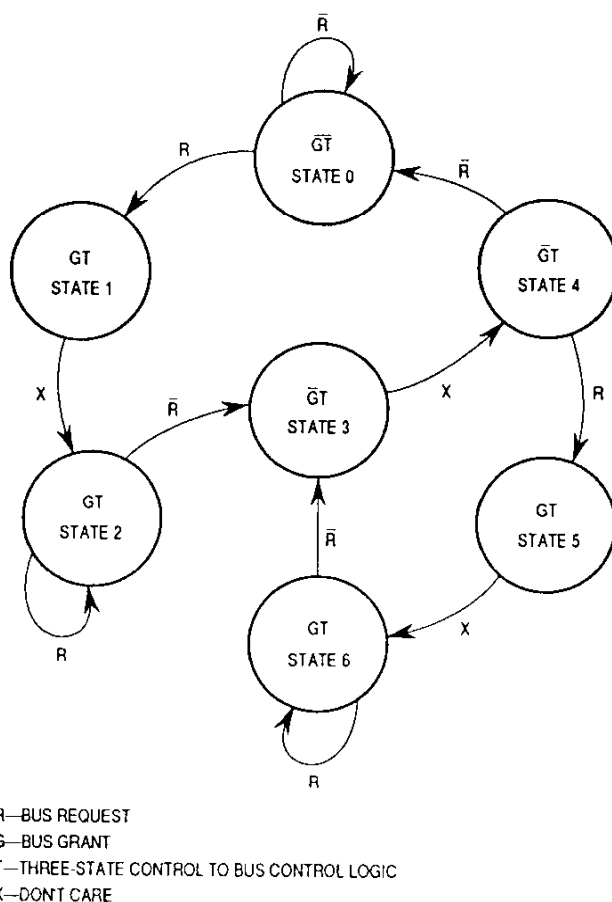
Figure 5-48. MC68EC020 Bus Arbitration State Diagram
