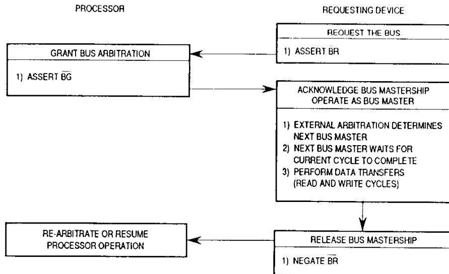
Figure 5-46. MC68EC020 Bus Arbitration Flowchart for Single Request
