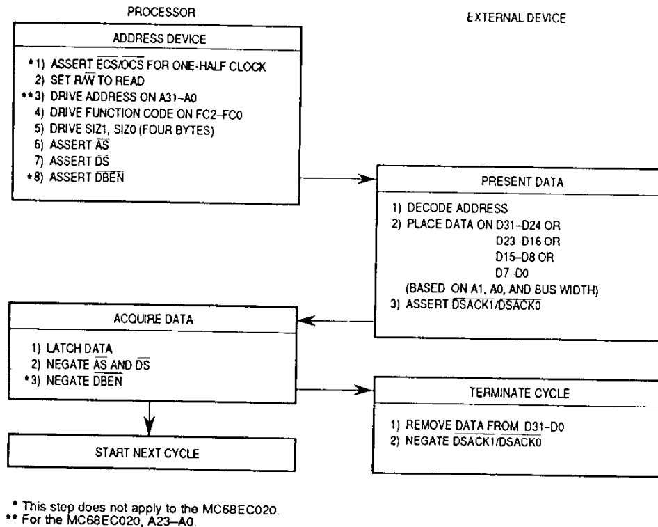
Figure 5-20. Byte Read Cycle Flowchart
