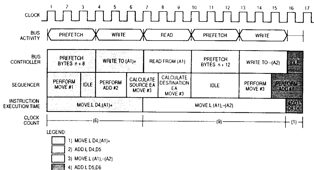
Figure 8-3. Processor Activity for Example 1
