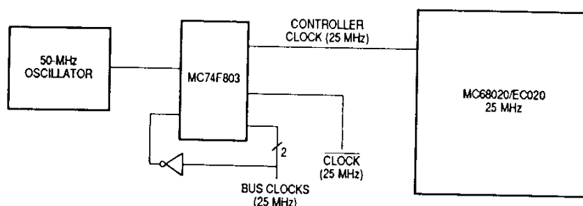
Figure 9-8. Alternate Clock Solution
