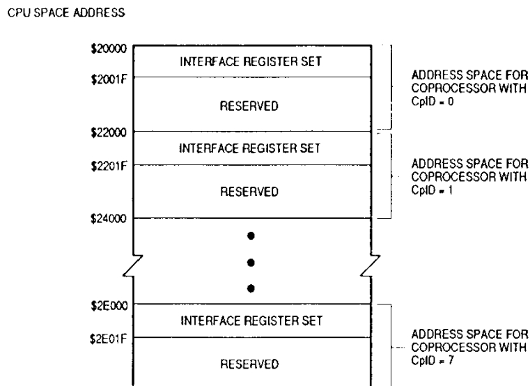
Figure 7-4. Coprocessor Address Map in MC68020/EC020 CPU Space
