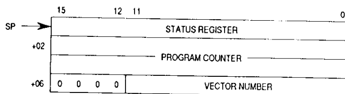
Figure 7-41. MC68020/EC020 Preinstruction Stack Frame
