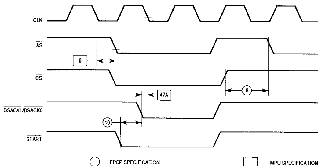
Figure 9-4. Bus Cycle Timing Diagram
