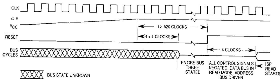
Figure 5-51. Initial Reset Operation Timing
