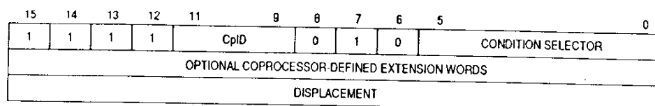
Figure 7-9. Branch on Coprocessor Condition Instruction Format (cpBcc.W)
