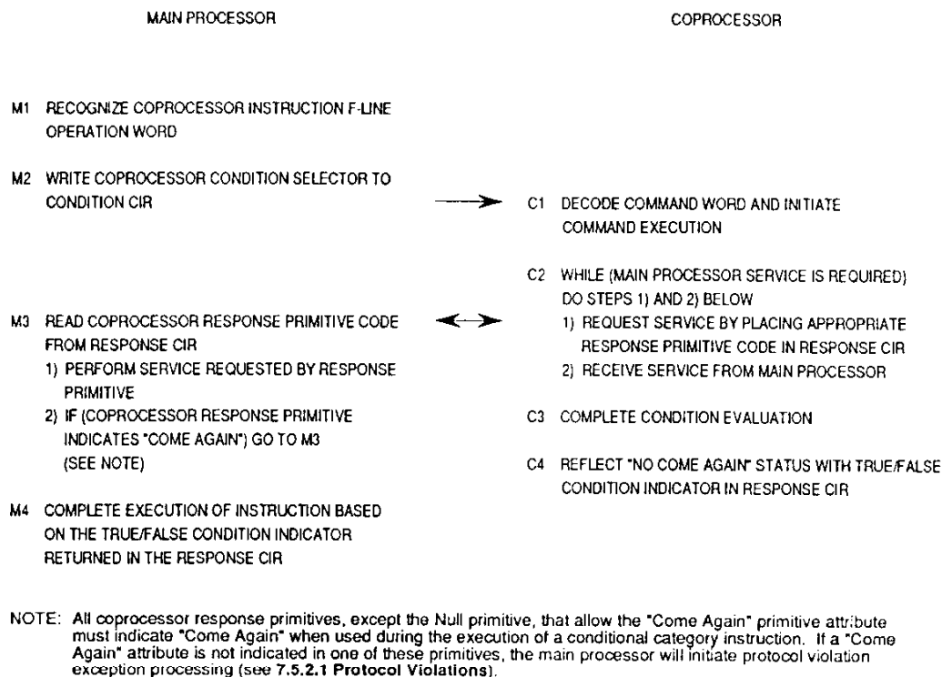
Figure 7-8. Coprocessor Interface Protocol for Conditional Category Instructions
