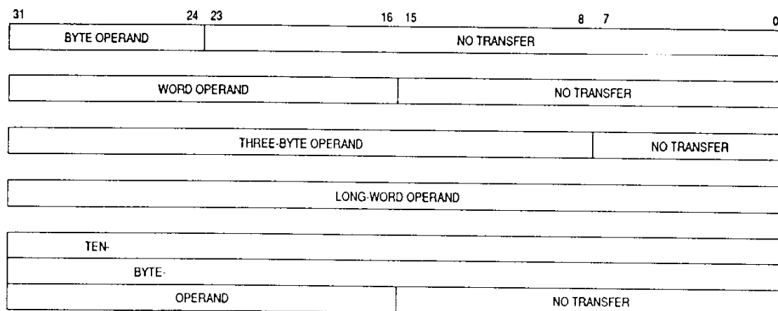
Figure 7-21. Operand Alignment for Operand CIR Accesses
