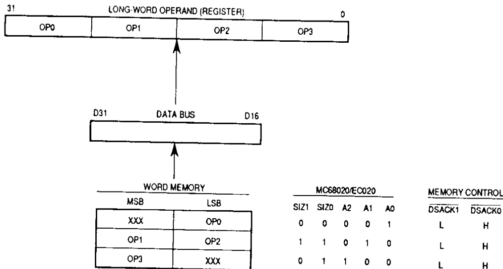
Figure 5-11. Misaligned Long-Word Operand Read from Word Port Example
