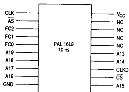
Figure 9-2. Chip Select Generation PAL
