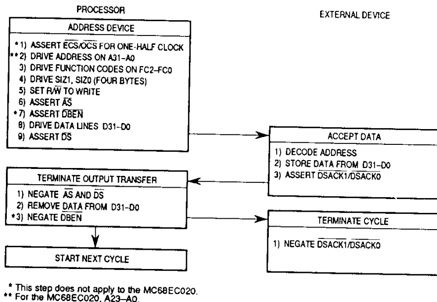
Figure 5-24. Write Cycle Flowchart
