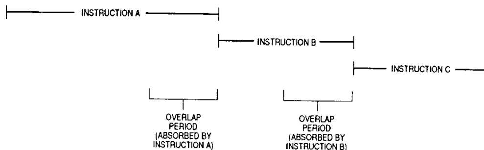
Figure 8-2. Instruction Execution for Instruction Timing Purposes
