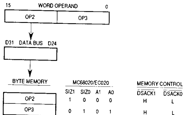
Figure 5-7. Word Operand Write to Byte Port Example
