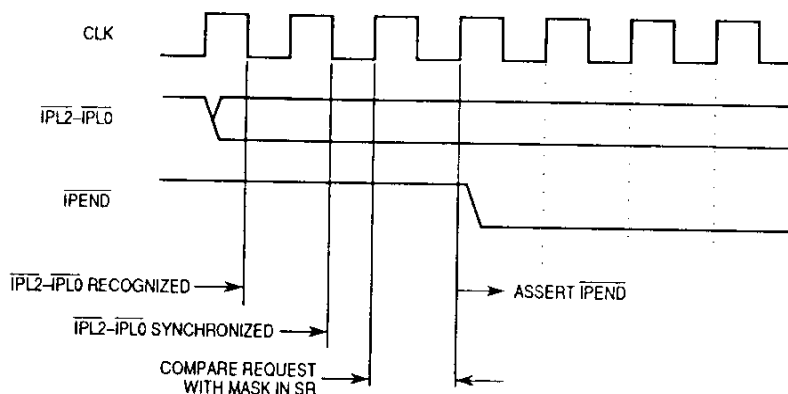
Figure 6-4. Assertion of \overline{IPEND} (MC68020 Only)
