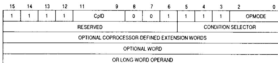
Figure 7-13. Trap on Coprocessor Condition Instruction Format (cpTRAPcc)
