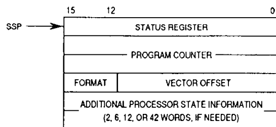
Figure 2-1. General Exception Stack Frame
