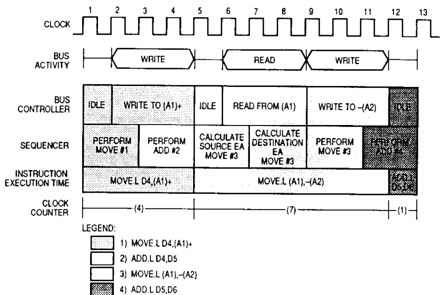
Figure 8-5. Processor Activity for Example 3
