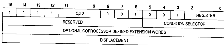
Figure 7-12. Test Coprocessor Condition, Decrement, and Branch Instruction Format (cpDBcc)
