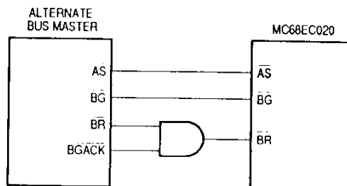
Figure 5-50. Interface for Three-Wire to Two-Wire Bus Arbitration
