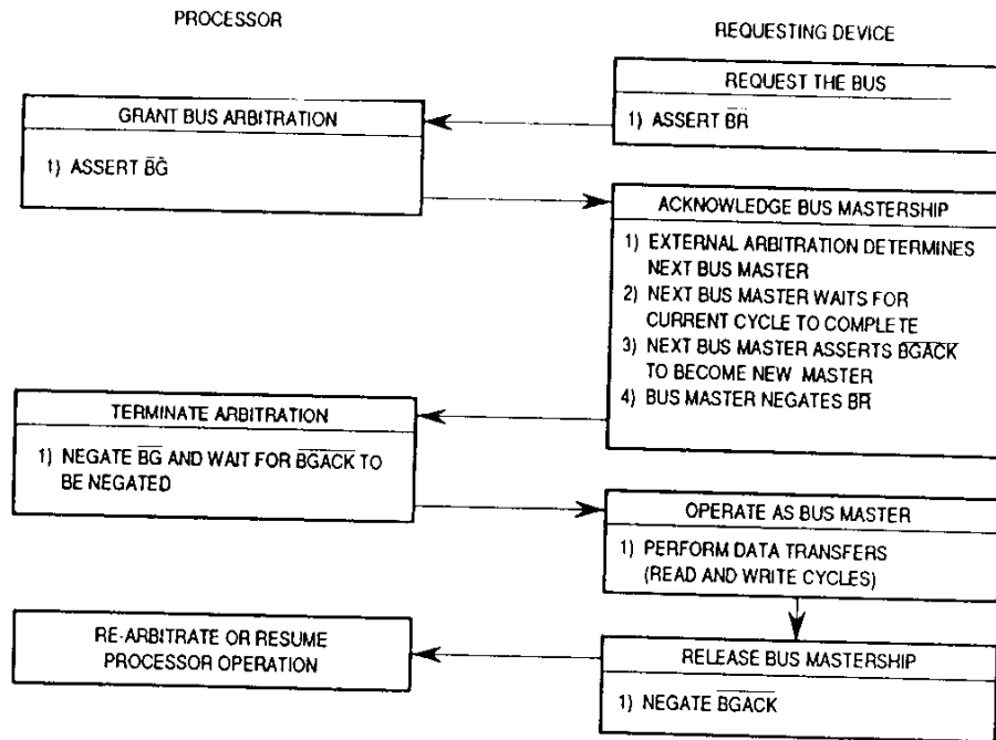
Figure 5-42. MC68020 Bus Arbitration Flowchart for Single Request
