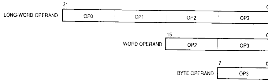
Figure 5-3. Internal Operand Representation
