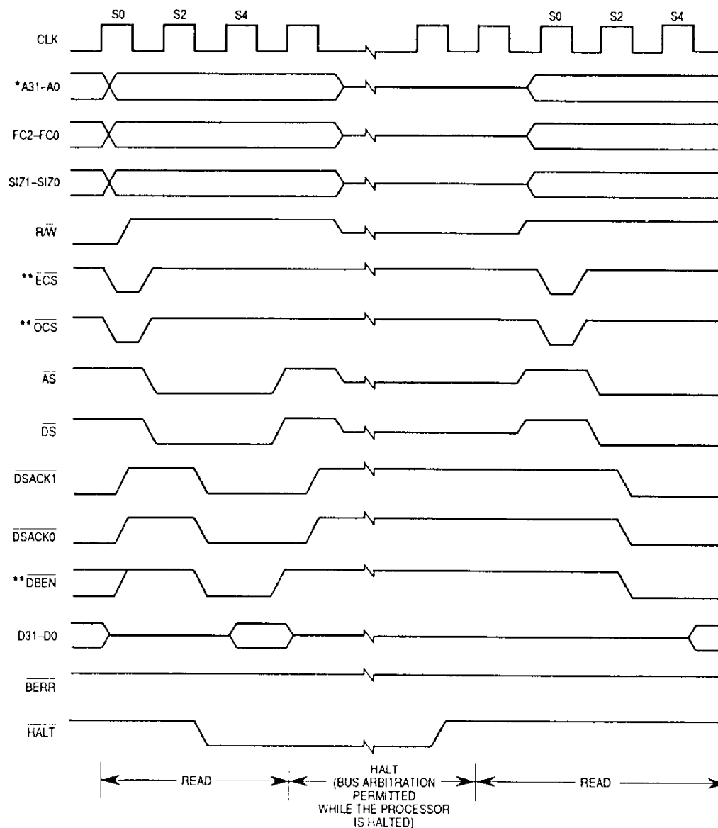
Figure 5-41. Halt Operation Timing
