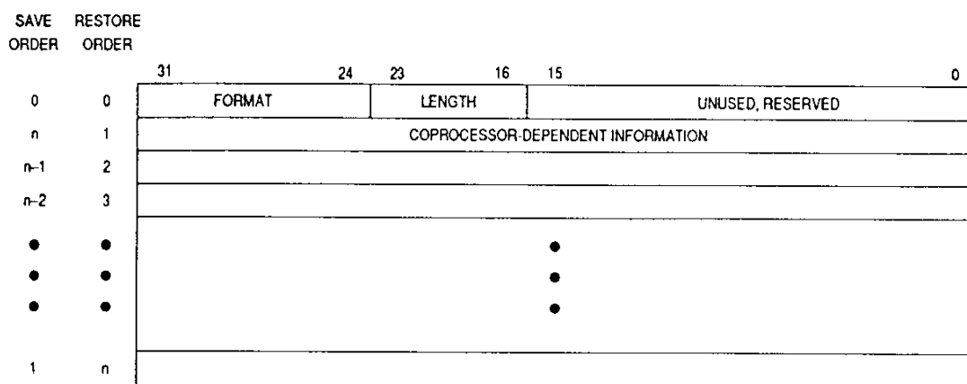
Figure 7-14. Coprocessor State Frame Format in Memory
