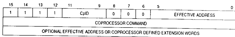
Figure 7-6. Coprocessor General Instruction Format (cpGEN)
