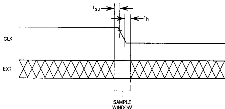
Figure 5-2. Input Sample Window
