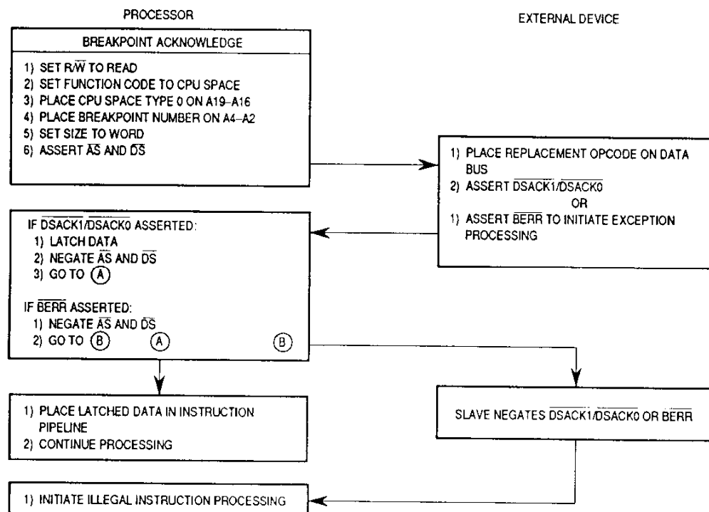
Figure 5-35. Breakpoint Acknowledge Cycle Flowchart
