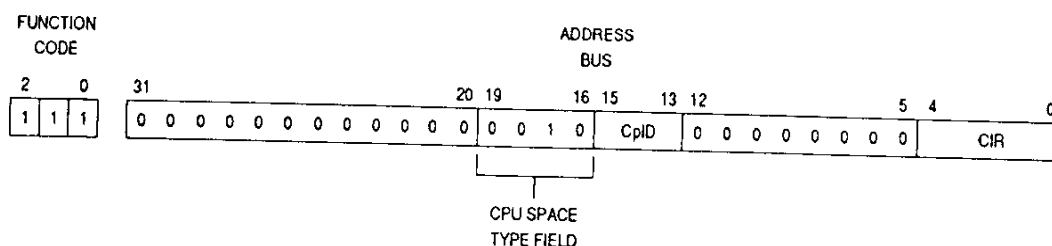
Figure 7-3. MC68020/EC020 CPU Space Address Encodings
