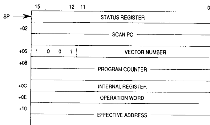
Figure 7-43. MC68020/EC020 Midinstruction Stack Frame
