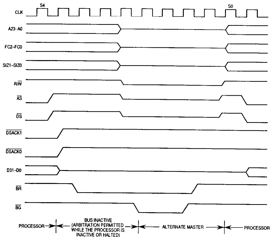
Figure 5-49. MC68EC020 Bus Arbitration Operation Timing—Bus Inactive
