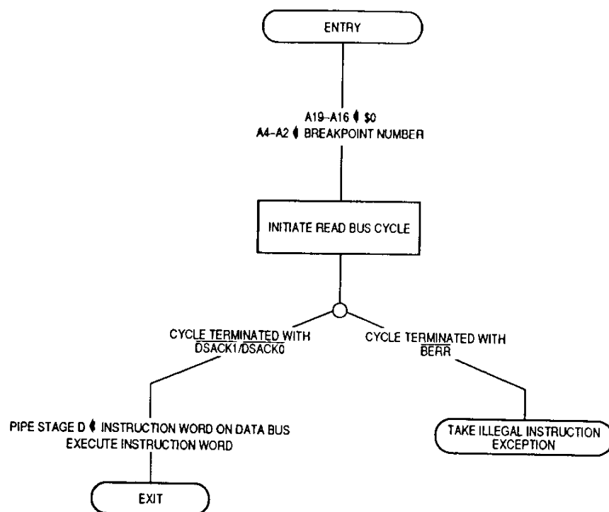
Figure 6-6. Breakpoint Instruction Flowchart
