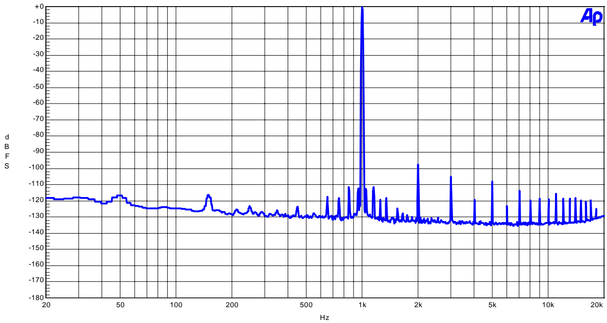
Figure 6. FFT Plot
