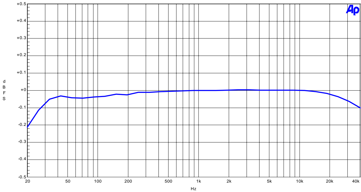
Figure 12. Frequency Response
