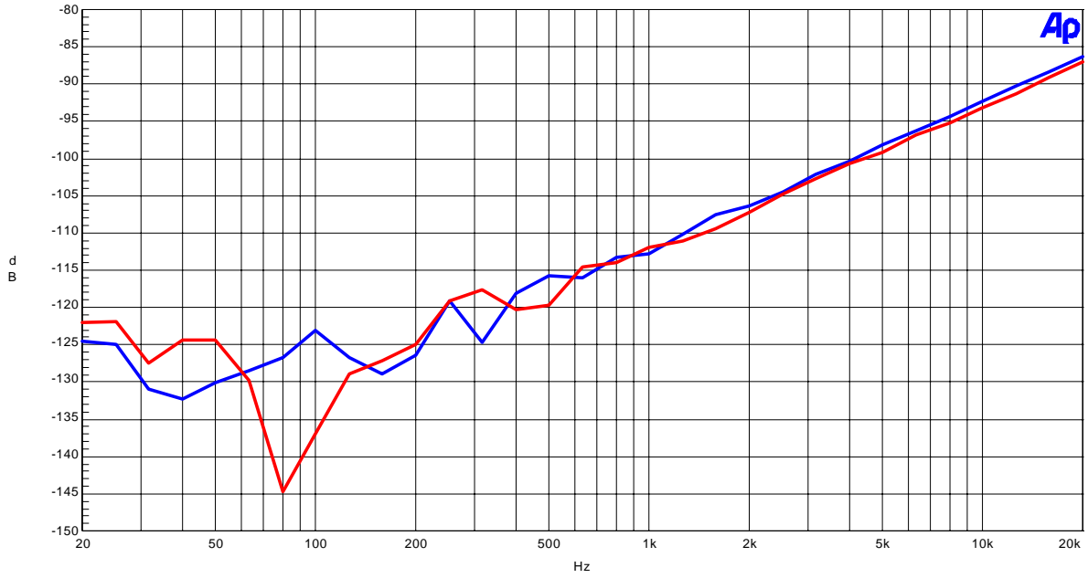
Figure 5. Crosstalk
