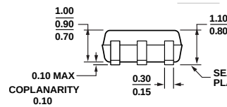
Figure 35. 5-Lead Thin Shrink Small Outline Transistor Package [SC70] (KS-5)
