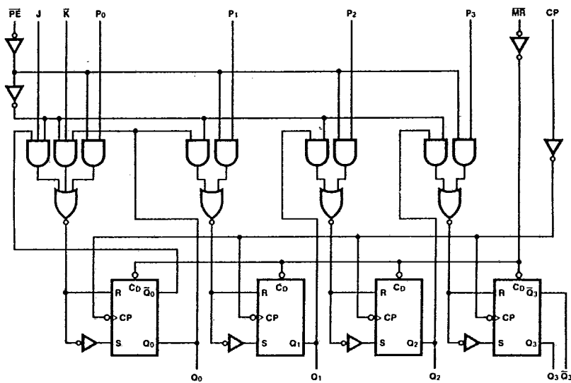
LOGIC DIAGRAM
