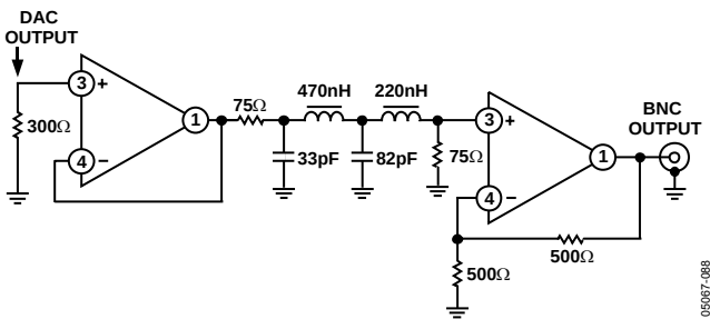
Figure 88. Example of Output Filter for HDTV, 2x Oversampling
