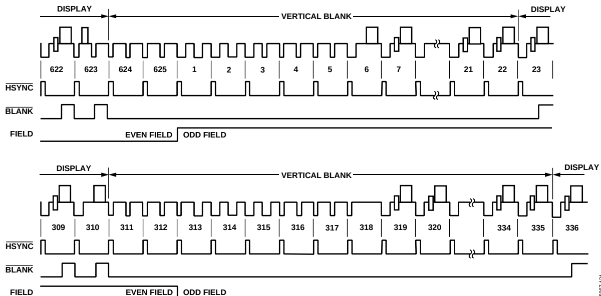
Figure 121. SD Timing Mode 3 (PAL)
