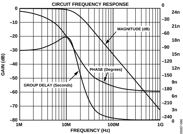
Figure 86. Filter Plot for Output Filter for SD, 16x Oversampling
