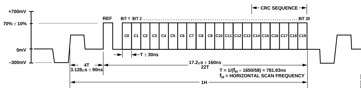
Figure 95. HDTV 720p CGMS Waveform
