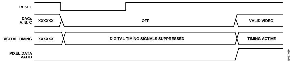
Figure 63. \overline{\text{RESET}} Timing Sequence
