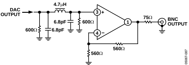
Figure 87. Example of Output Filter for PS, 8x Oversampling
