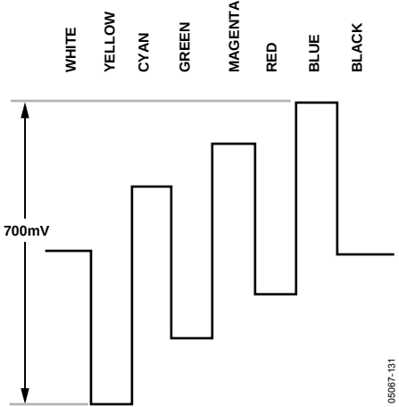
Figure 131. Pb Levels—NTSC
