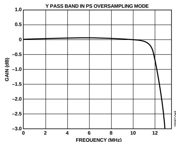
Figure 23. PS—Y 8x Oversampling Filter (Pass Band)
