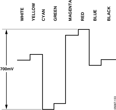
Figure 132. Pb Levels—PAL
