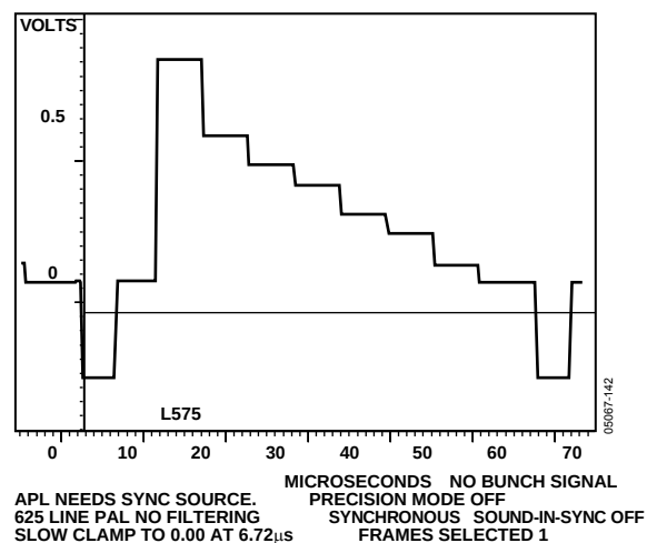
Figure 142. PAL Luma
