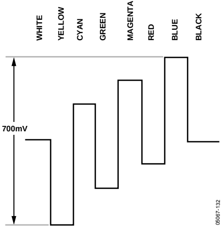
Figure 132. Pb Levels—PAL
