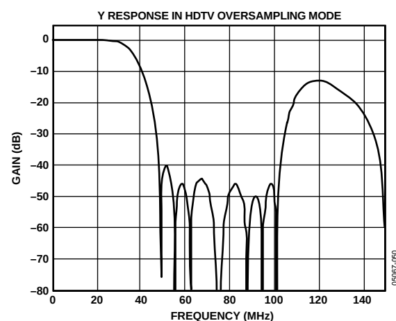
Figure 25. HDTV—Y 2x Oversampling Filter
