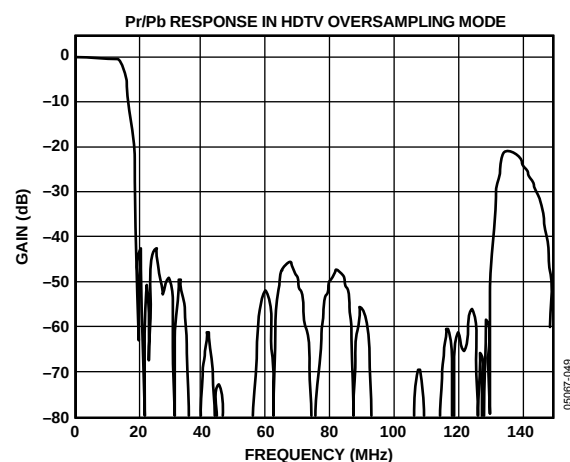
Figure 24. HDTV—UV 2x Oversampling Filter
