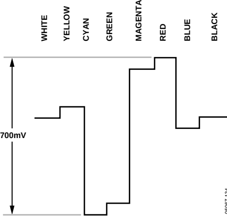
Figure 134. Pr Levels—PAL
