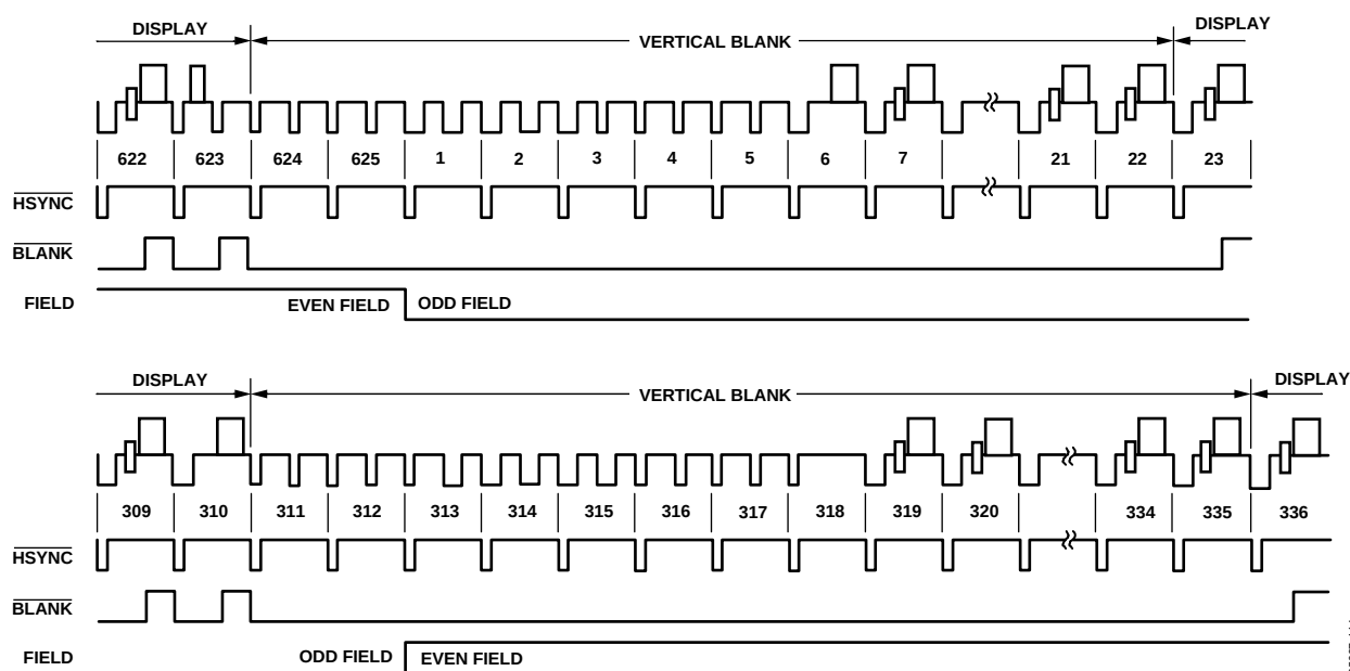
Figure 114. SD Slave Mode 1 (PAL)
