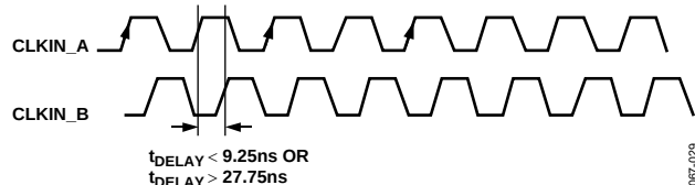
Figure 53. Clock Phase with Two Input Clocks
