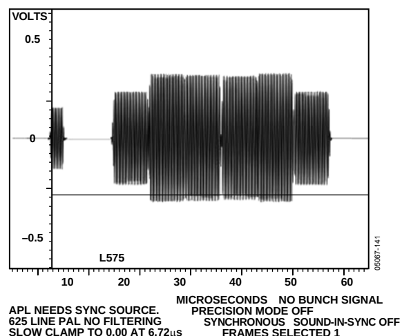
Figure 141. PAL Chroma
