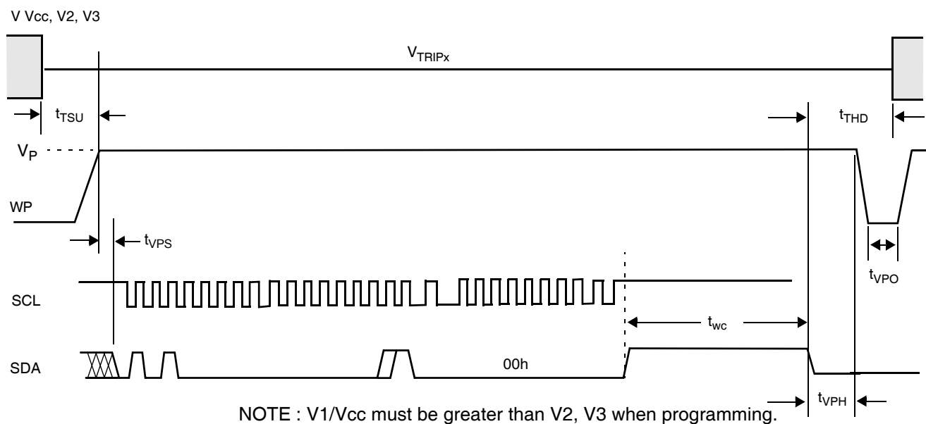
Figure 29. DCP “Wiper Position” Timing
