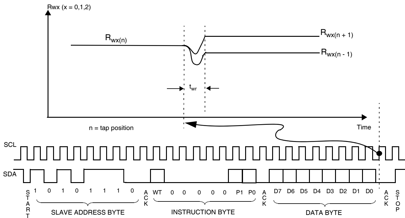
Figure 29. DCP “Wiper Position” Timing
