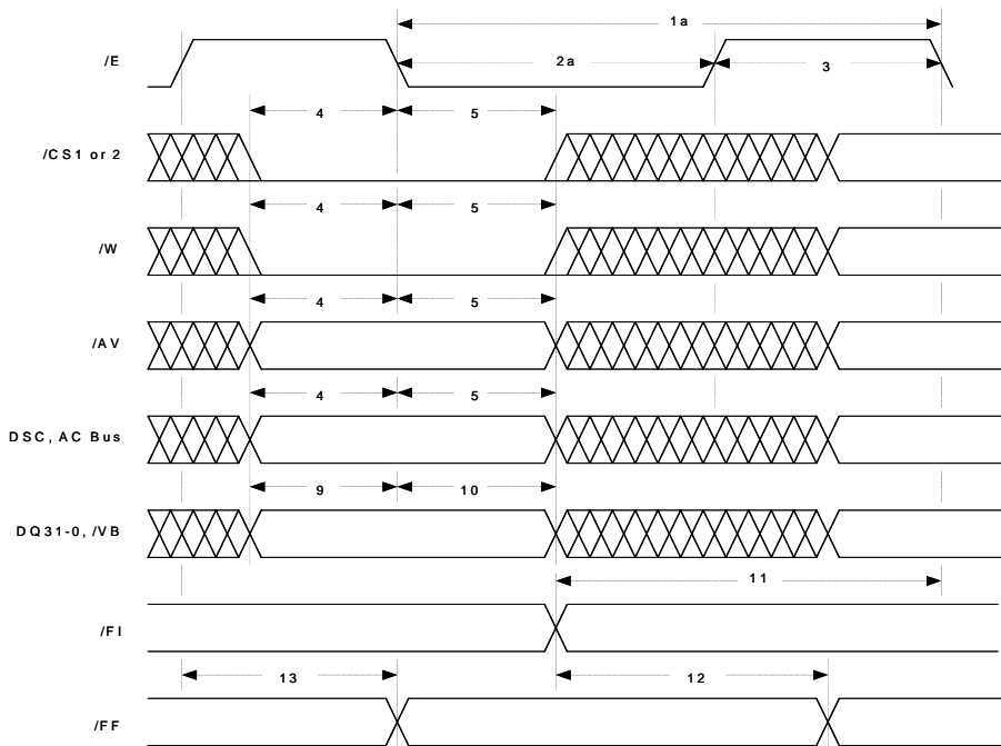
Figure 8: Write Cycle
