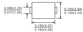
DO-214AA(SMB)
