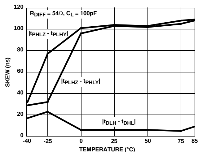
FIGURE 24. RS-485, DRIVER SKEW vs TEMPERATURE (MEDIUM DATA RATE, QFN ONLY)
