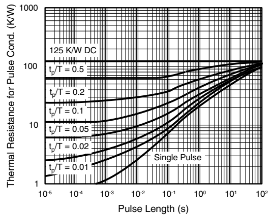
Fig. 8 - Thermal Response
