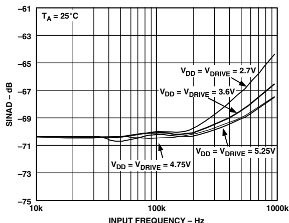
TPC 2. SINAD vs. Input Frequency
