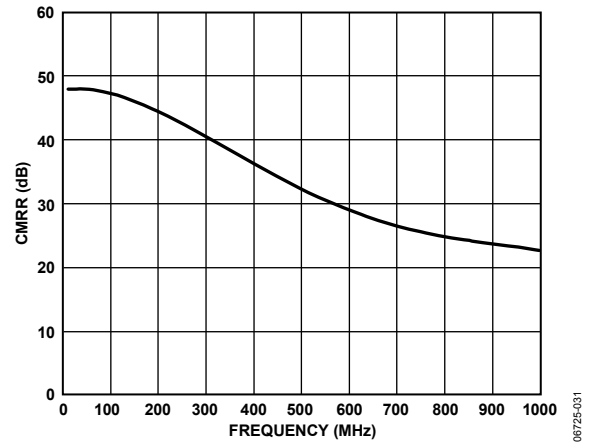
Figure 32. Common-Mode Rejection Ratio vs. Frequency
