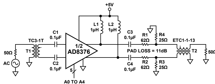
Figure 46. Test Circuit for Distortion, Gain, and Noise
