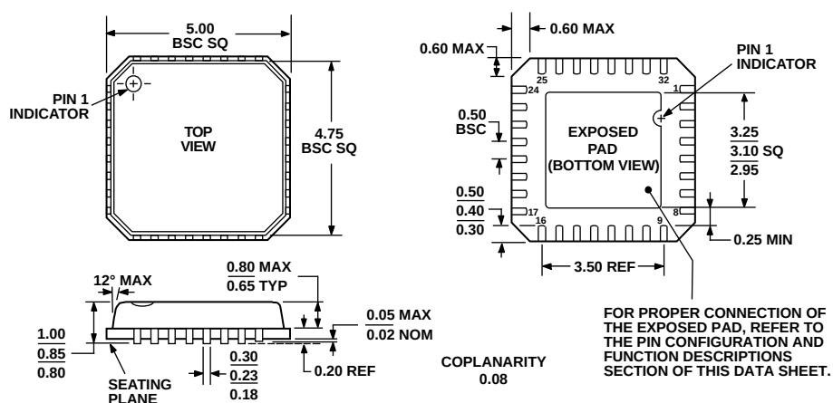
Figure 52. 32-Lead Lead Frame Chip Scale Package [LFCSP_VQ] 5 mm × 5 mm Body, Very Thin Quad (CP-32-2) Dimensions shown in millimeters
