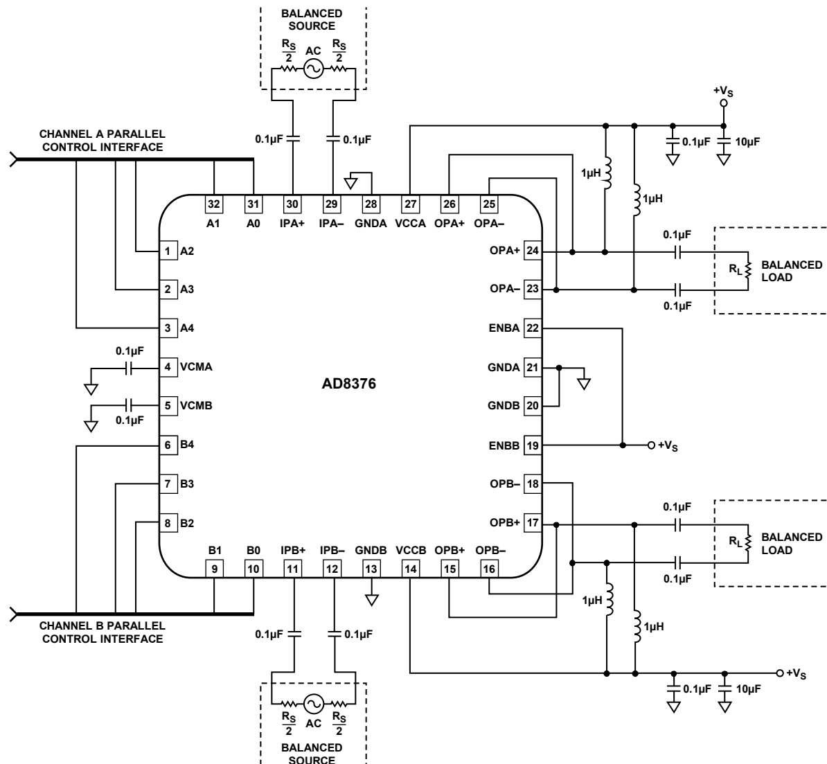
Figure 36. Basic Connections
