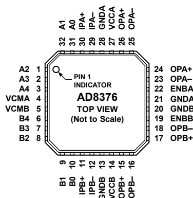
Figure 3. 32-Lead LFCSP
