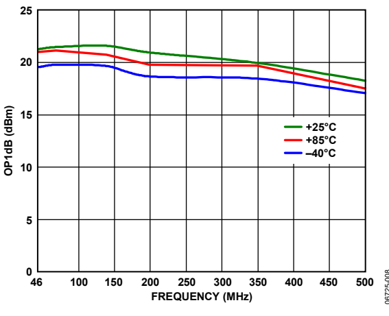
Figure 9. P1dB vs. Frequency at Maximum Gain, Three Temperatures
