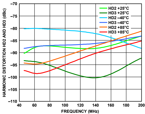
Figure 18. Harmonic Distortion vs. Frequency, Three Temperatures, V_{OUT} = 2 V_{p-p}
