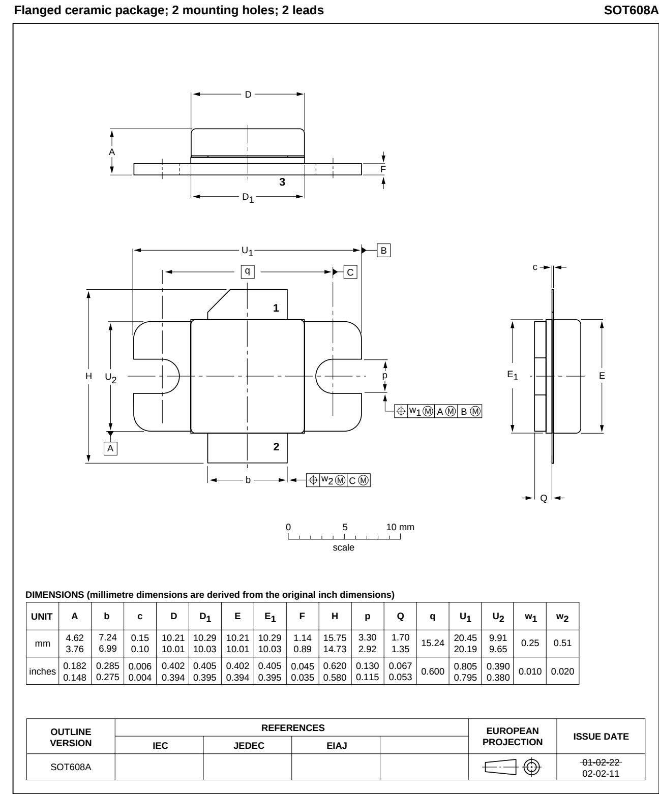
Fig 12. Package outline SOT608A
