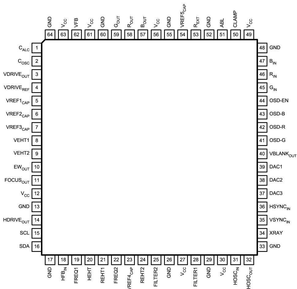
Figure 1. 64-Pin Non-Exposed DAP - TQFP Package See Package Number PAG0064A Exposed DAP – HTQFP Package See Package Number PAP0064A
