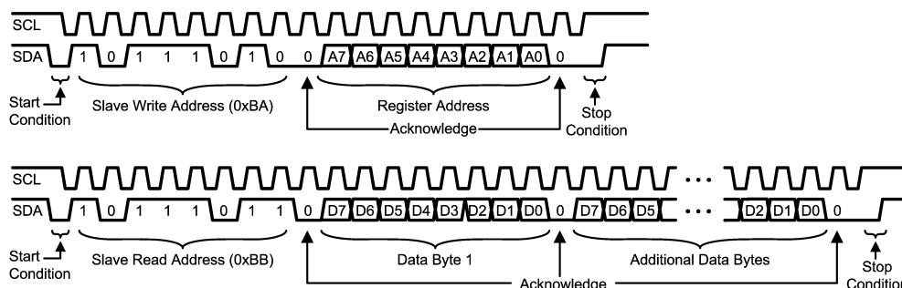
Figure 10. I²C Compatible Read Sequence
