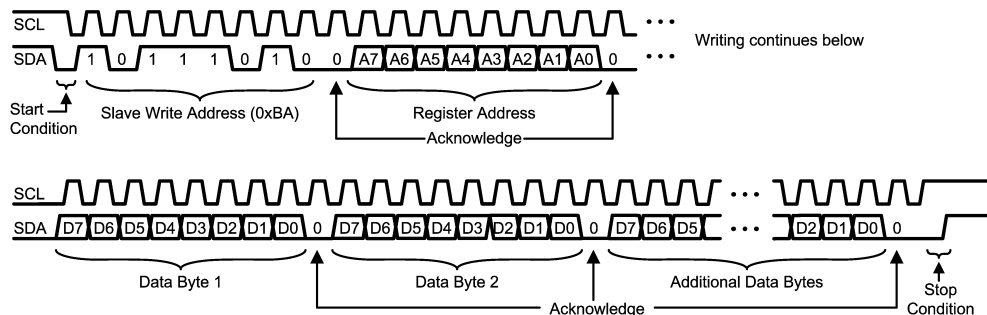
Figure 9. I²C Compatible Write Sequence
