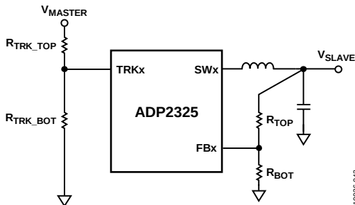
Figure 47. Voltage Tracking
