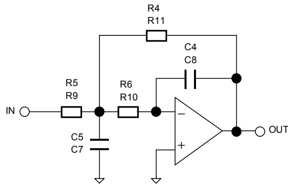
Fig.35 LPF and echo system gain
