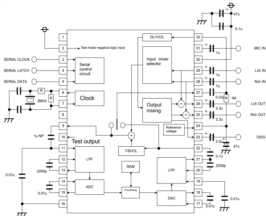
Fig.30 Application circuit
