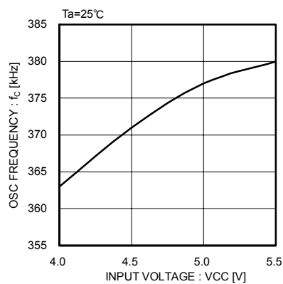
Fig.2 Oscillation frequency
