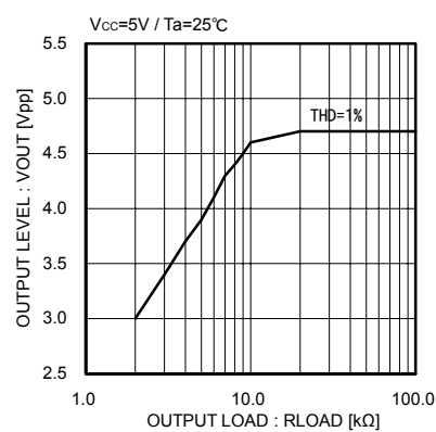
Fig.12 Delay side output load drive characteristic
