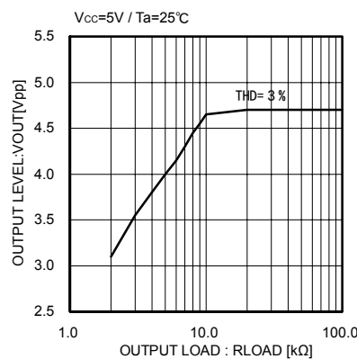
Fig.9 Through side output load drive characteristic
