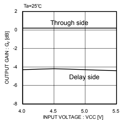
Fig.3 Total gain characteristic
