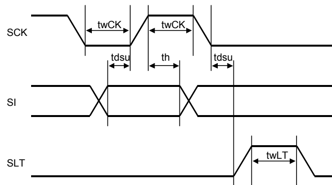
Fig.34 Serial timing
