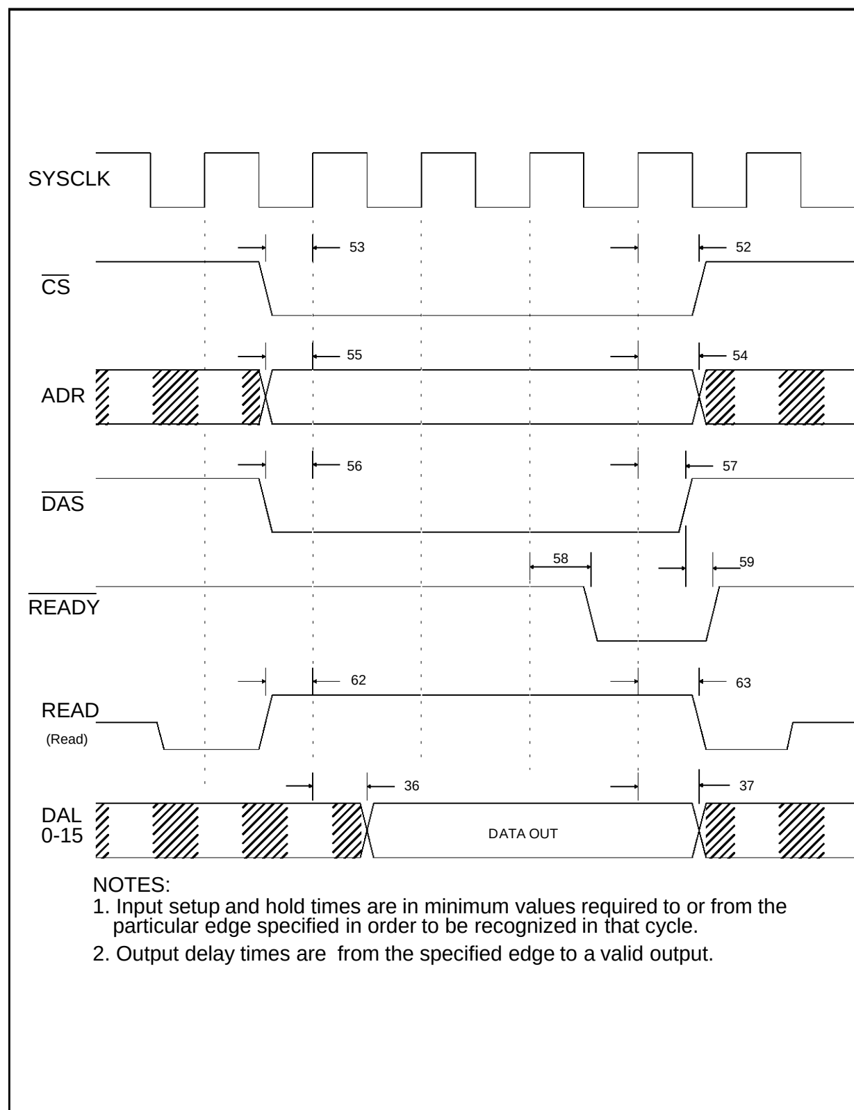
Figure 9: MK50H27 BUS Slave Timing Diagram (Read)
