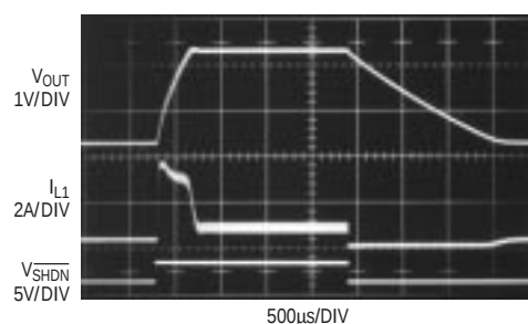
Figure 11. 5V Boost Converter of Figure 1. Start-Up from 3V Input into 5Ω Load
