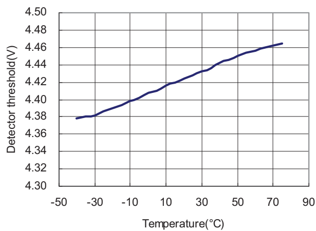
Detector threshold=4.4V
