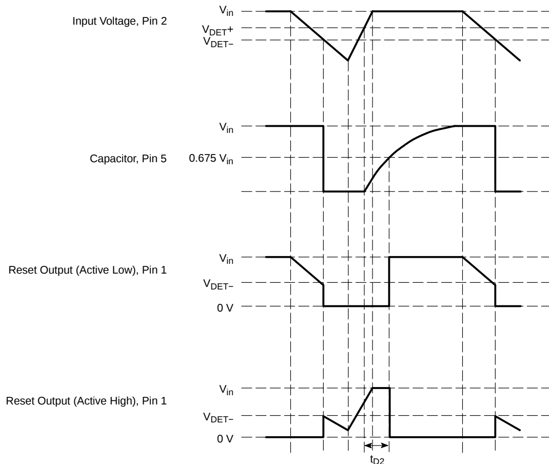
Timing Waveforms
