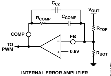
Figure 19. Compensation Using the ESR Zero
