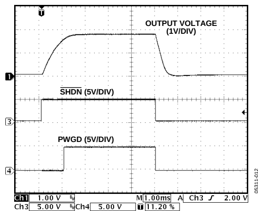
Figure 11. Power-On Response
