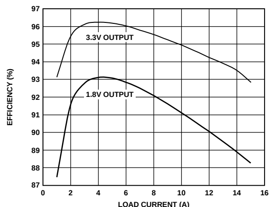
Figure 1. Efficiency vs. Load Current, 5 V Input
