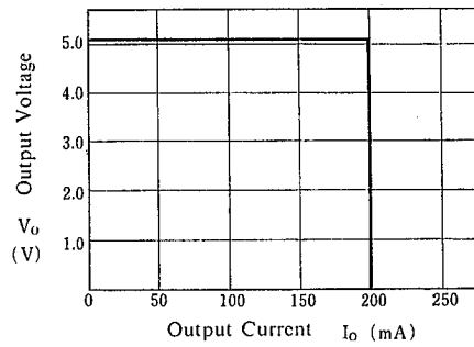
NJM2930F05/L05 Load Characteristics ( V_{IN}=14V , T_j=25^\circ\text{C} )
