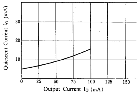
NJM2930F05 Output Current vs. Quiescent Current ( V_{IN}=14V , T_j=25^\circ\text{C} )
