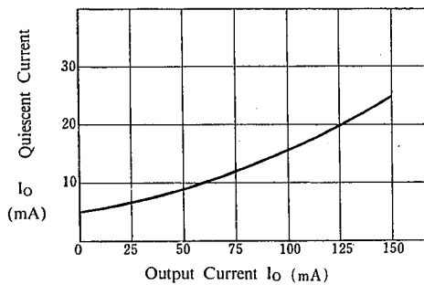
NJM2930L05 Output Current vs. Quiescent Current ( V_{IN}=14V , T_j=25^\circ\text{C} )
