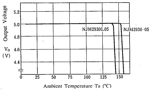
NJM2939F05/L05 Thermal Shutdown ( V_{IN}=14V , I_o=50\text{mA} )
