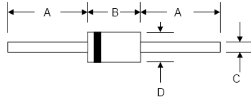
DO-15
