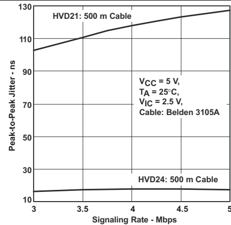
Figure 8. SN65HVD2[1,4] Peak-to-Peak Jitter vs Signaling Rate
