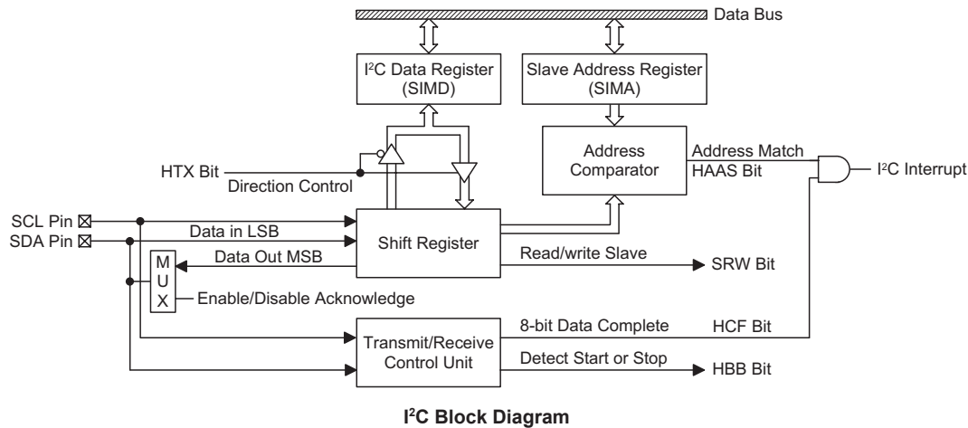
I 2 C Block Diagram
