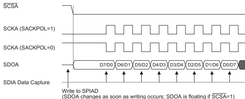
SPIA Slave Mode Timing – SACKEG= 0
