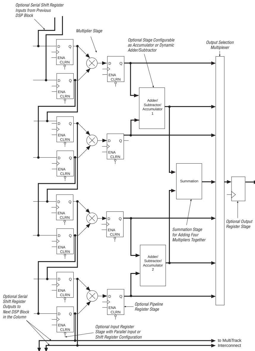
Figure 2–58. DSP Block Diagram for 18 \times 18 -Bit Configuration
