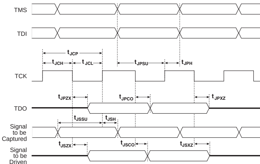
Figure 4–14. Stratix II GX JTAG Waveforms.
