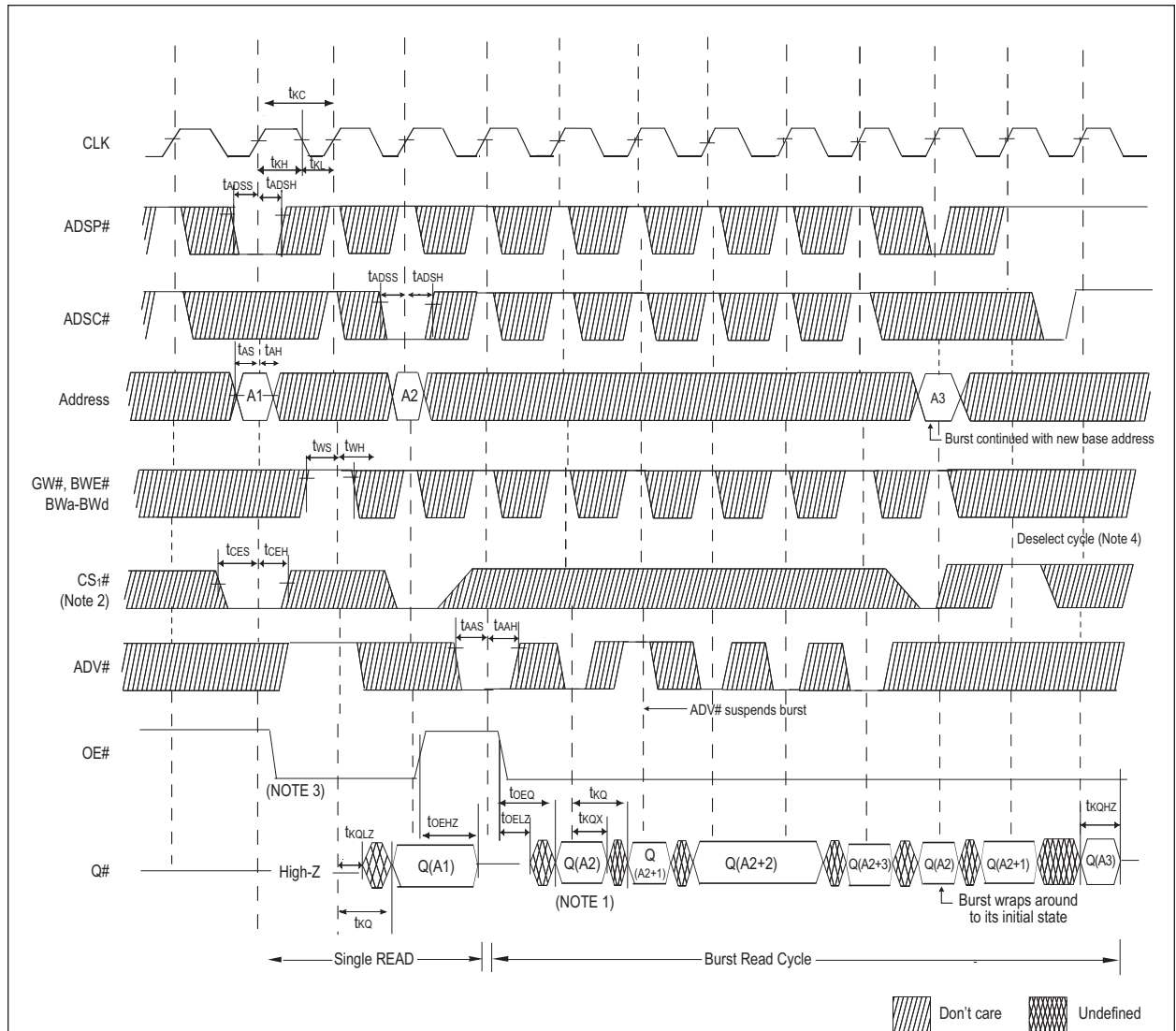
FIGURE 2 – READ TIMING 3
