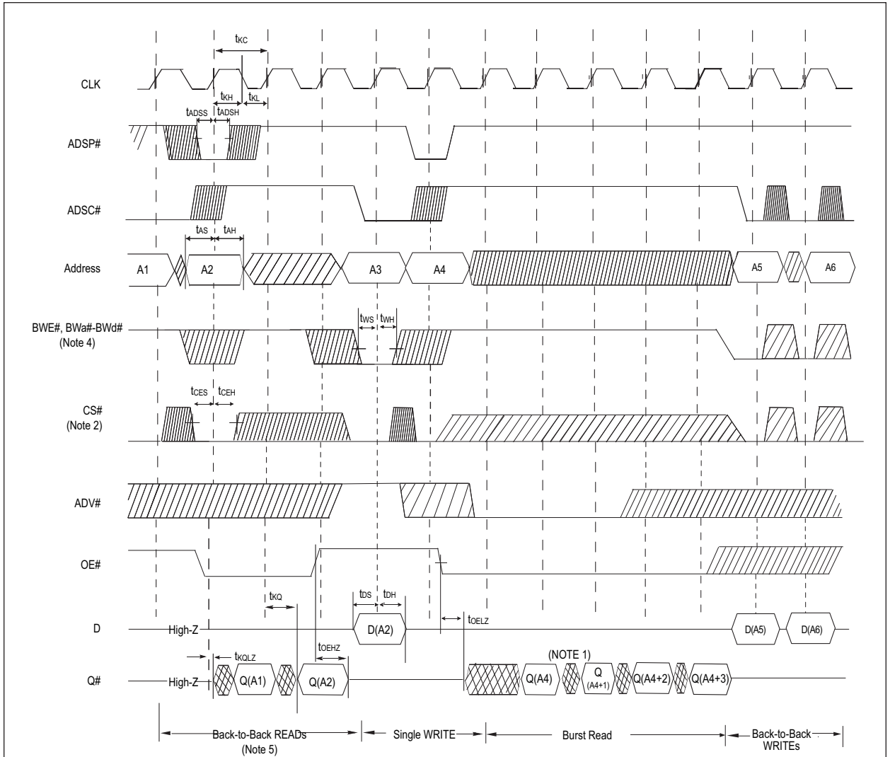
FIGURE 5 – READ/WRITE TIMING 3
