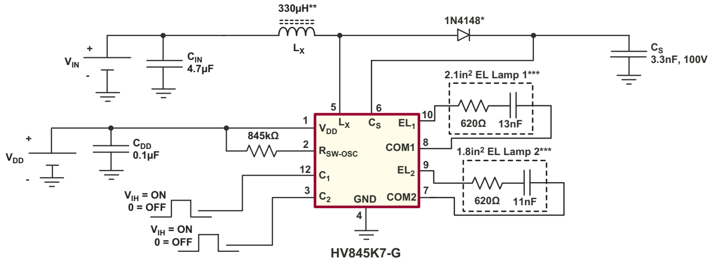
Figure 1 - Test Circuit
