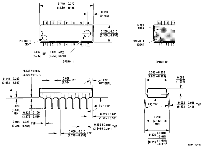
14-Lead Molded Dual-In-Line Package (N) Order Number DM7495N NS Package Number N14A
