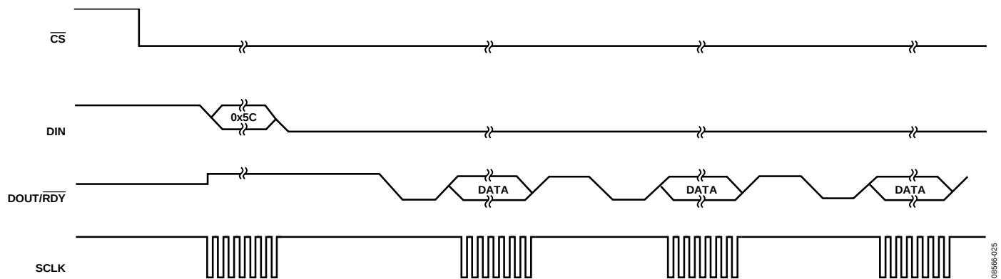
Figure 26. Continuous Read
