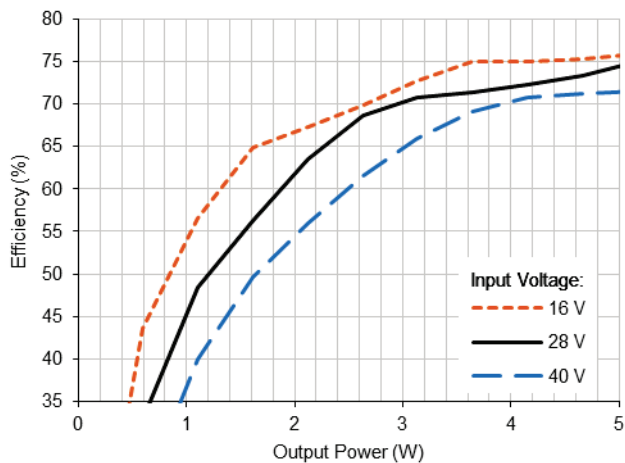
4.1.3 VHR5-2812S Efficiency (%) vs. Output Power (W)
