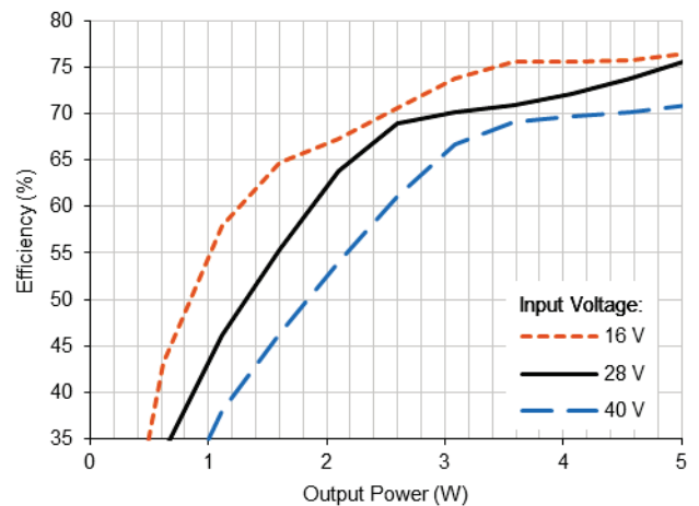
4.1.4 VHR5-2815S Efficiency (%) vs. Output Power (W)
