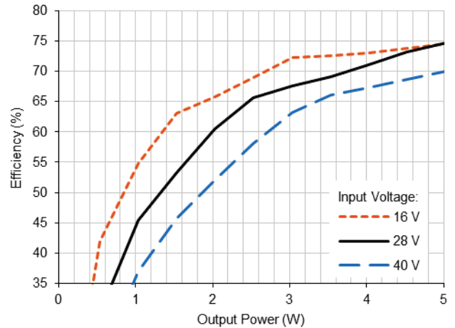
4.1.2 VHR5-2805S Efficiency (%) vs. Output Power (W)
