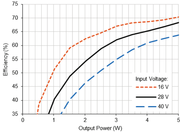
4.1.1 VHR5-283R3S Efficiency (%) vs. Output Power (W)
