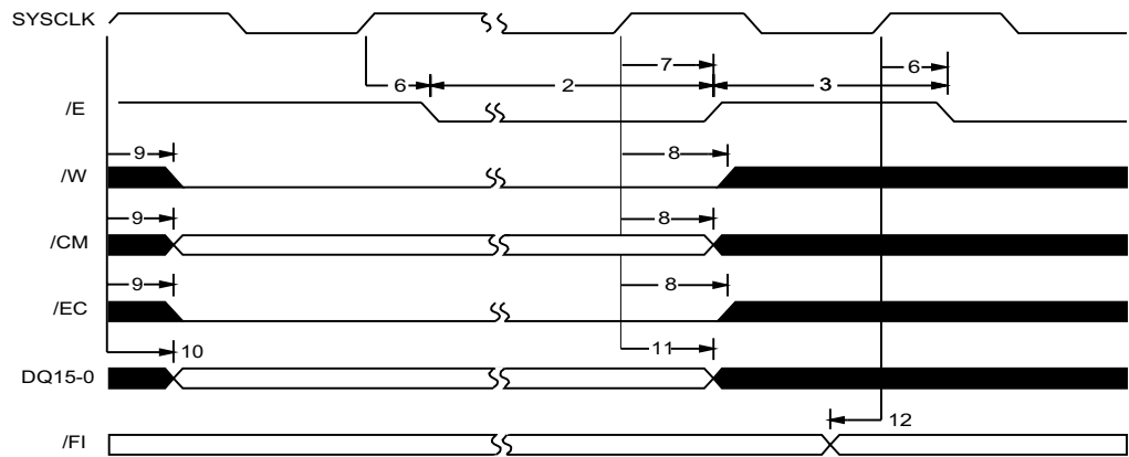
Figure 14: Timing Diagram for LANCAM: Write
