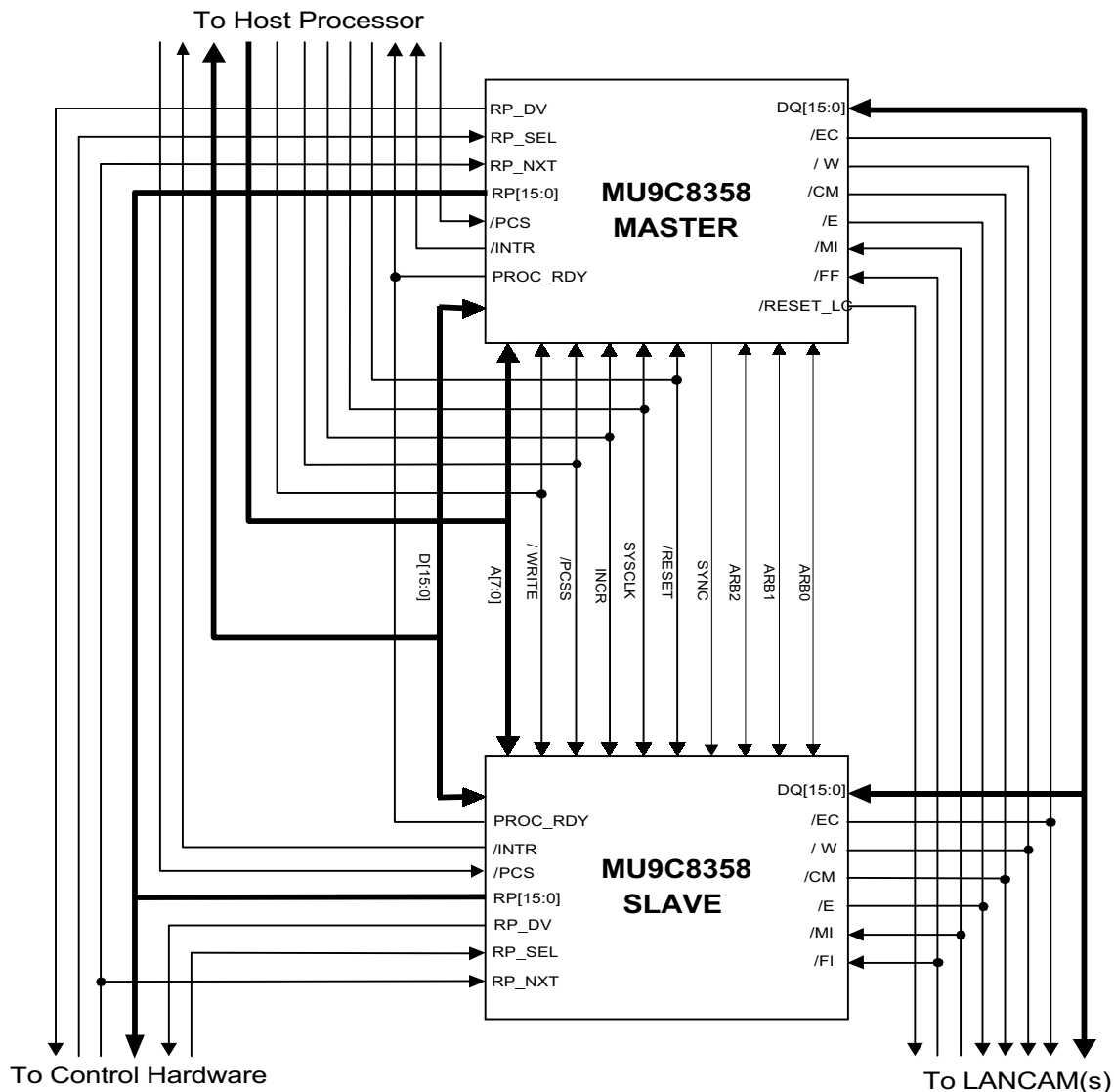
Figure 7: Cascading Two MU9C8358 Components
