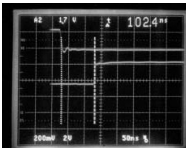
Actual oscilloscope photo showing 6.5 to 13.5 GHz step in 103 nanoseconds
