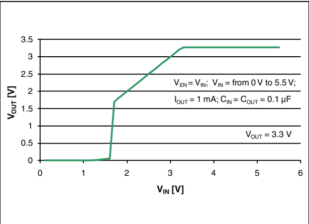
Figure 10. Output voltage vs. input voltage ( V_{OUT} = 3.3\text{ V} )
