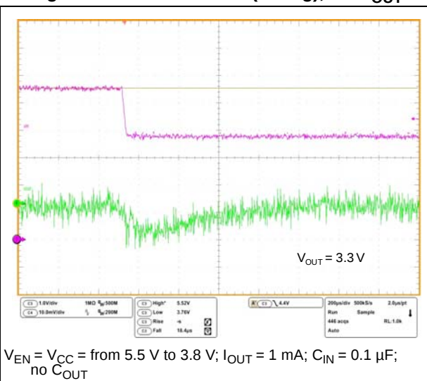
Figure 16. Line transient (falling), no C OUT
