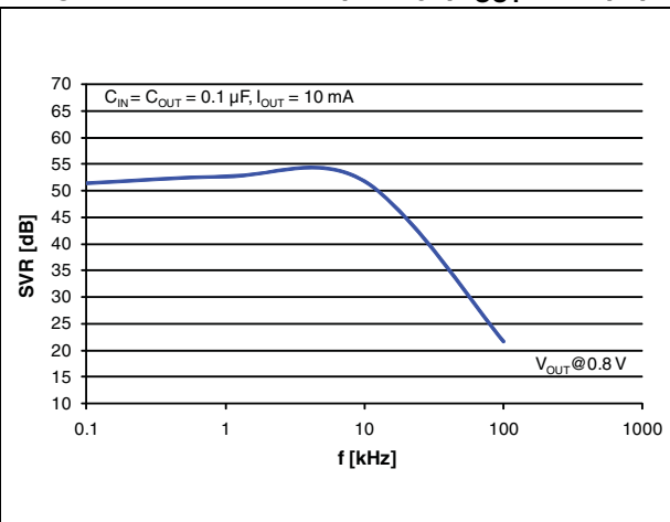
Figure 12. SVR vs. frequency (C OUT = 0.1 μF)
