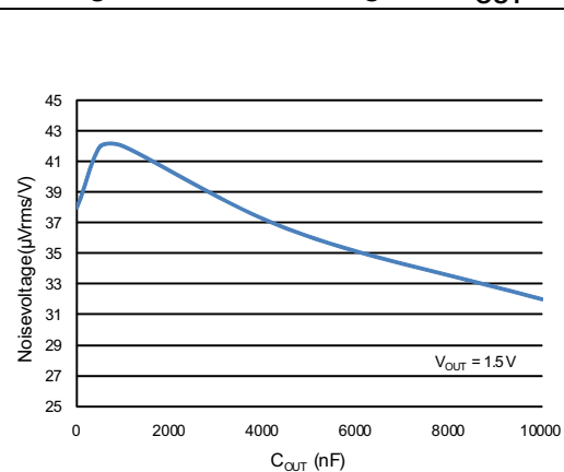
Figure 14. Noise voltage vs. C OUT
