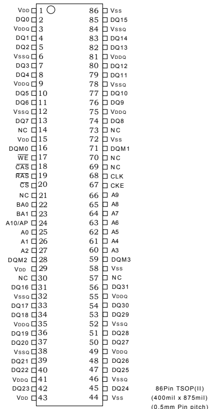
Top View
